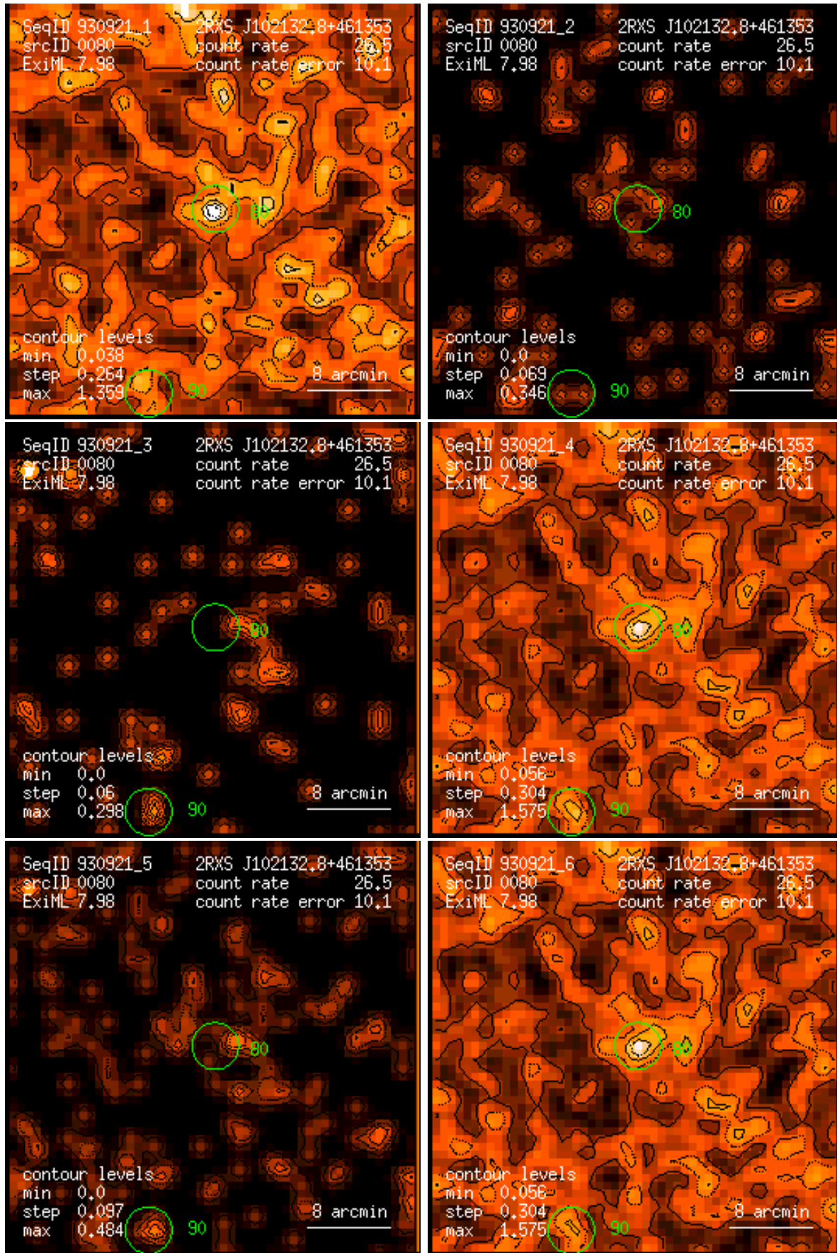
Figure 80: RASS 930921: detection 0080: band rate images, Gaussian filter: (1) PSPC channels 11 – 41, (2) 52 – 90, (3) 91 – 201, (4) 11 – 235, (5) 52 – 201, (6) 11 – 201. Broad band rates in counts/ks. Band rate contour levels in counts/ks/arcmin 2 .
