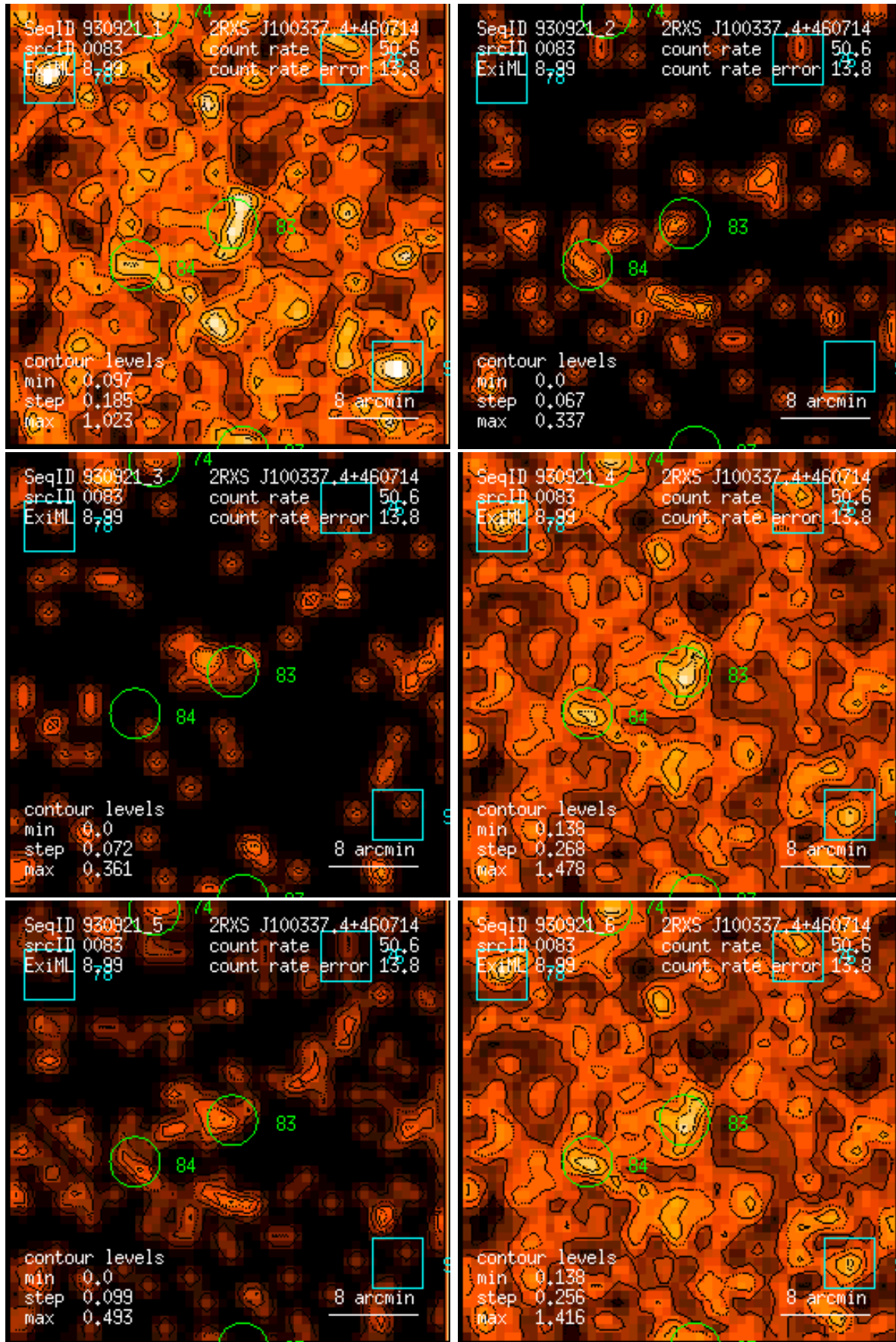
Figure 83: RASS 930921: detection 0083: band rate images, Gaussian filter: (1) PSPC channels 11 – 41, (2) 52 – 90, (3) 91 – 201, (4) 11 – 235, (5) 52 – 201, (6) 11 – 201. Broad band rates in counts/ks. Band rate contour levels in counts/ks/arcmin 2 .
