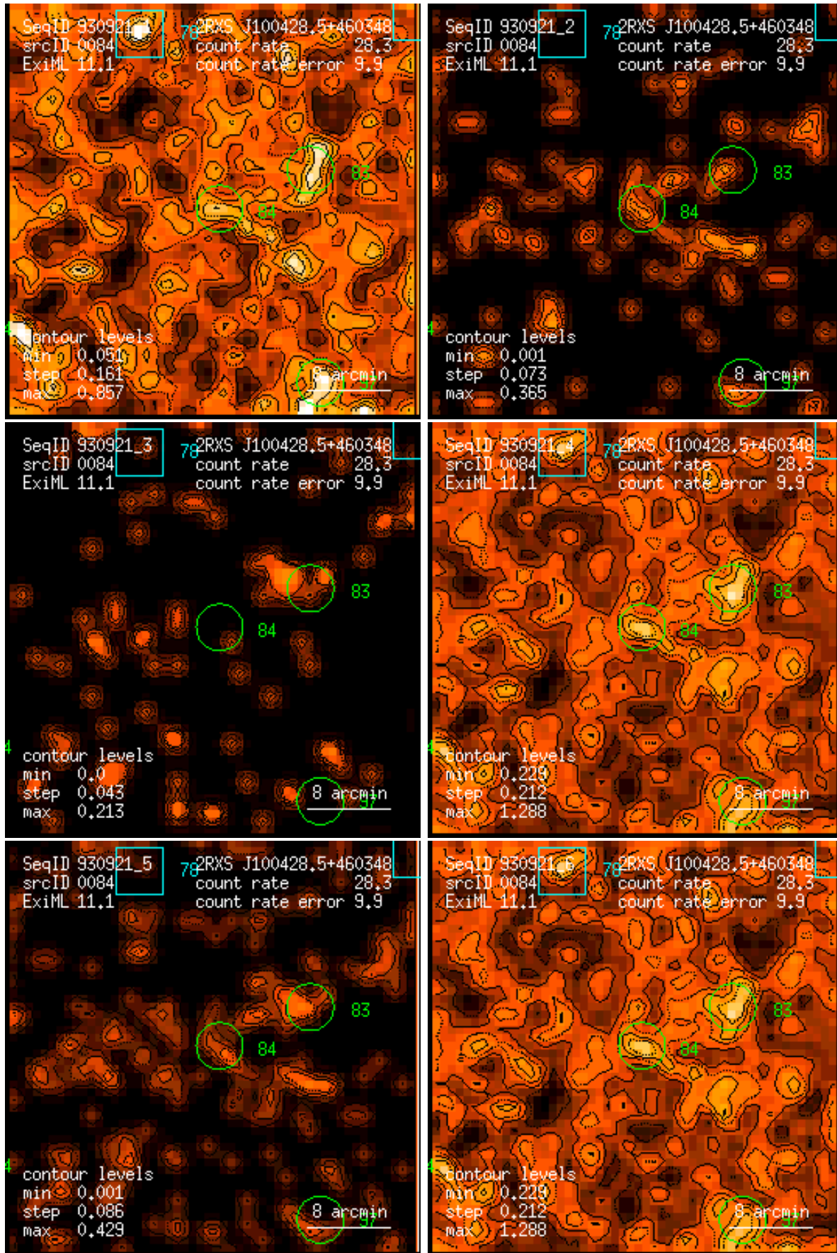
Figure 84: RASS 930921: detection 0084: band rate images, Gaussian filter: (1) PSPC channels 11 – 41, (2) 52 – 90, (3) 91 – 201, (4) 11 – 235, (5) 52 – 201, (6) 11 – 201. Broad band rates in counts/ks. Band rate contour levels in counts/ks/arcmin 2 .
