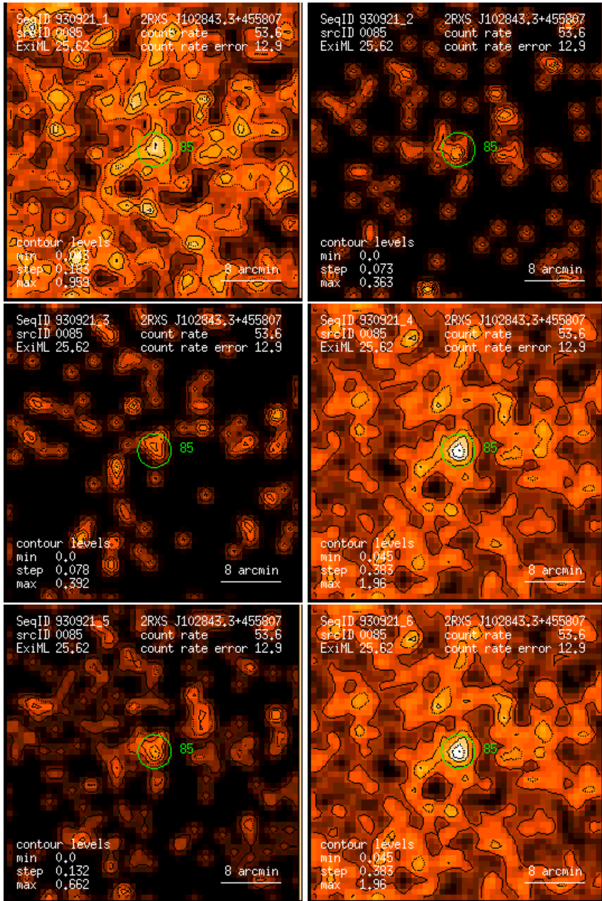
Figure 85: RASS 930921: detection 0085: band rate images, Gaussian filter: (1) PSPC channels 11 – 41, (2) 52 – 90, (3) 91 – 201, (4) 11 – 235, (5) 52 – 201, (6) 11 – 201. Broad band rates in counts/ks. Band rate contour levels in counts/ks/arcmin 2 .
