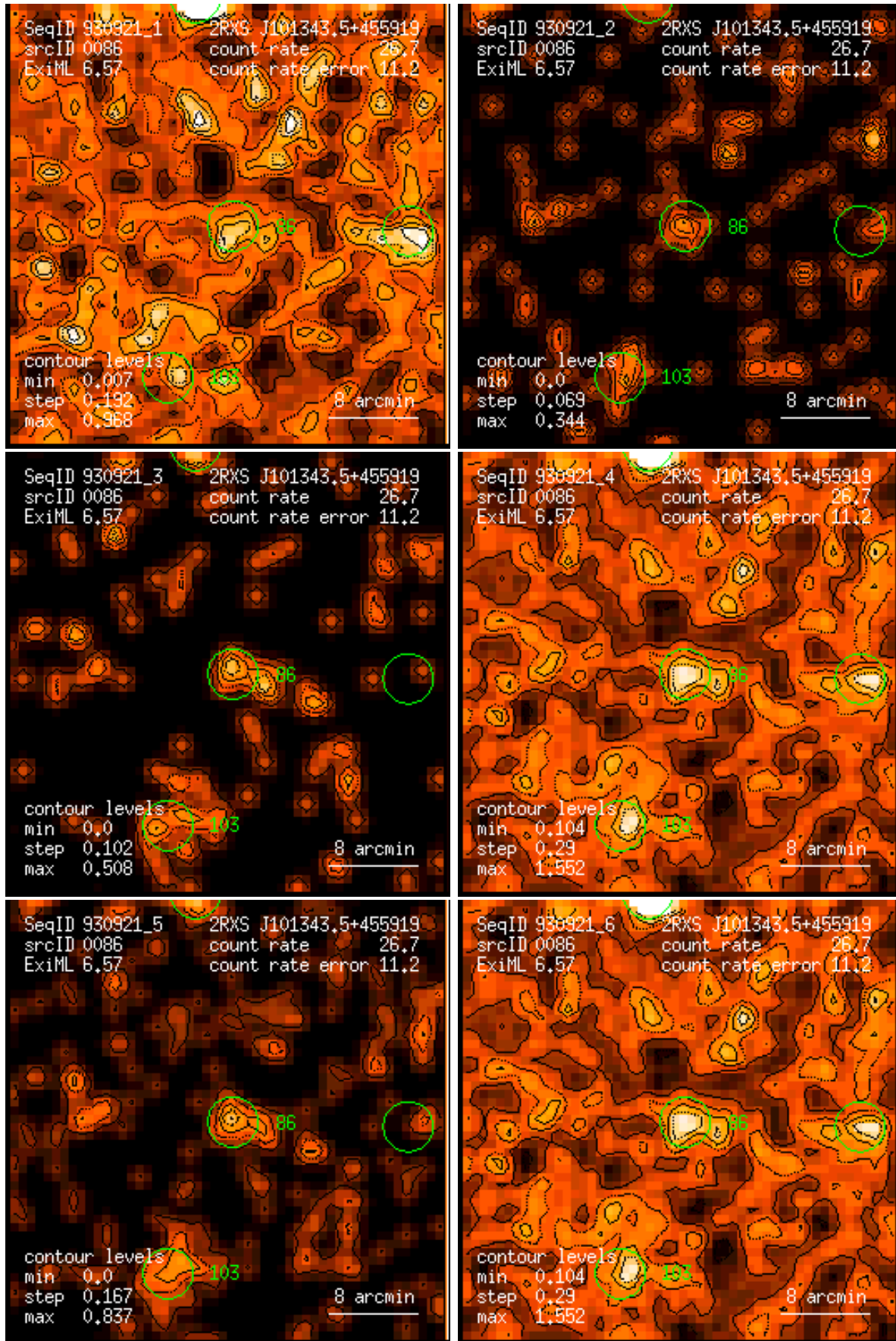
Figure 86: RASS 930921: detection 0086: band rate images, Gaussian filter: (1) PSPC channels 11 – 41, (2) 52 – 90, (3) 91 – 201, (4) 11 – 235, (5) 52 – 201, (6) 11 – 201. Broad band rates in counts/ks. Band rate contour levels in counts/ks/arcmin 2 .
