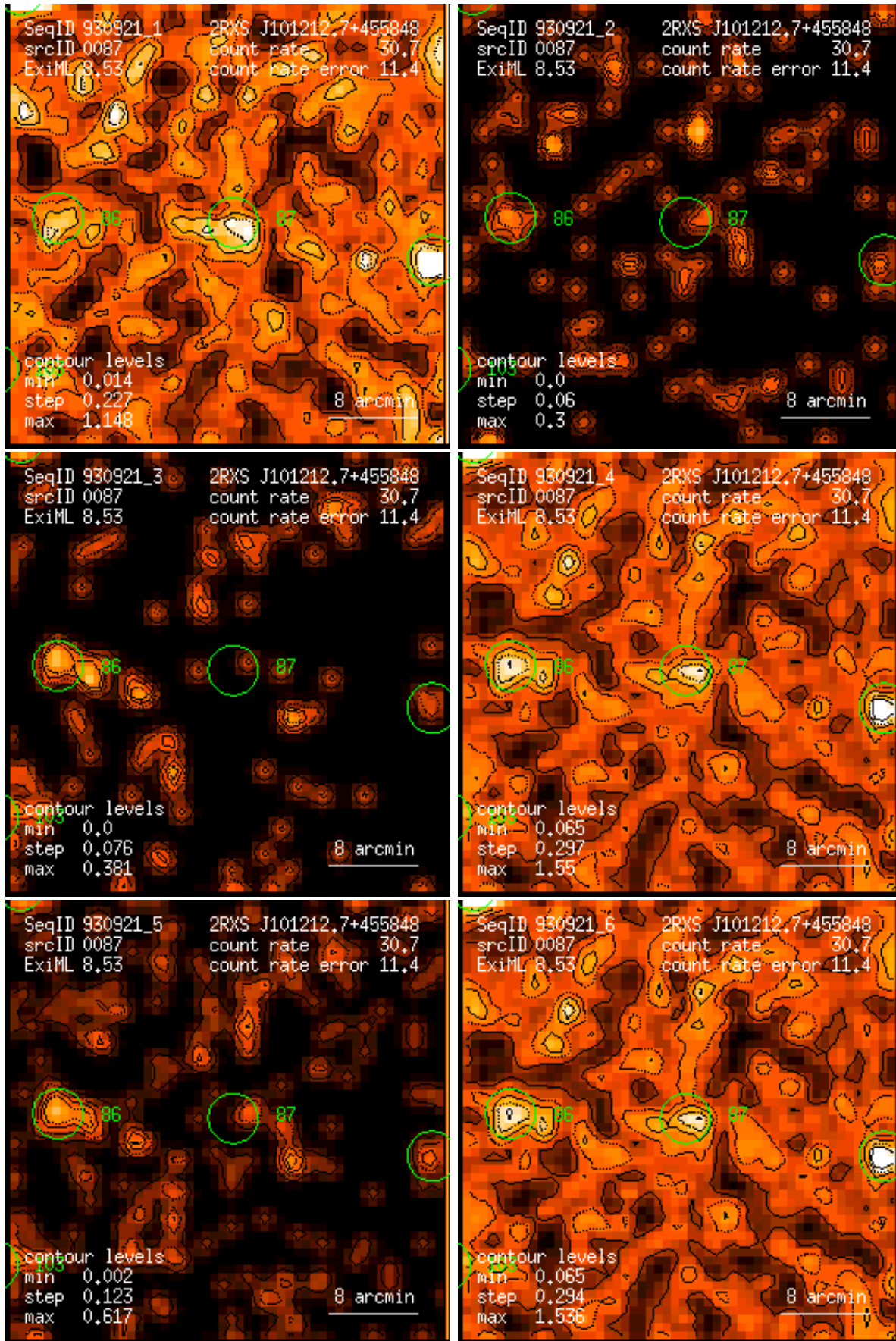
Figure 87: RASS 930921: detection 0087: band rate images, Gaussian filter: (1) PSPC channels 11 – 41, (2) 52 – 90, (3) 91 – 201, (4) 11 – 235, (5) 52 – 201, (6) 11 – 201. Broad band rates in counts/ks. Band rate contour levels in counts/ks/arcmin 2 .
