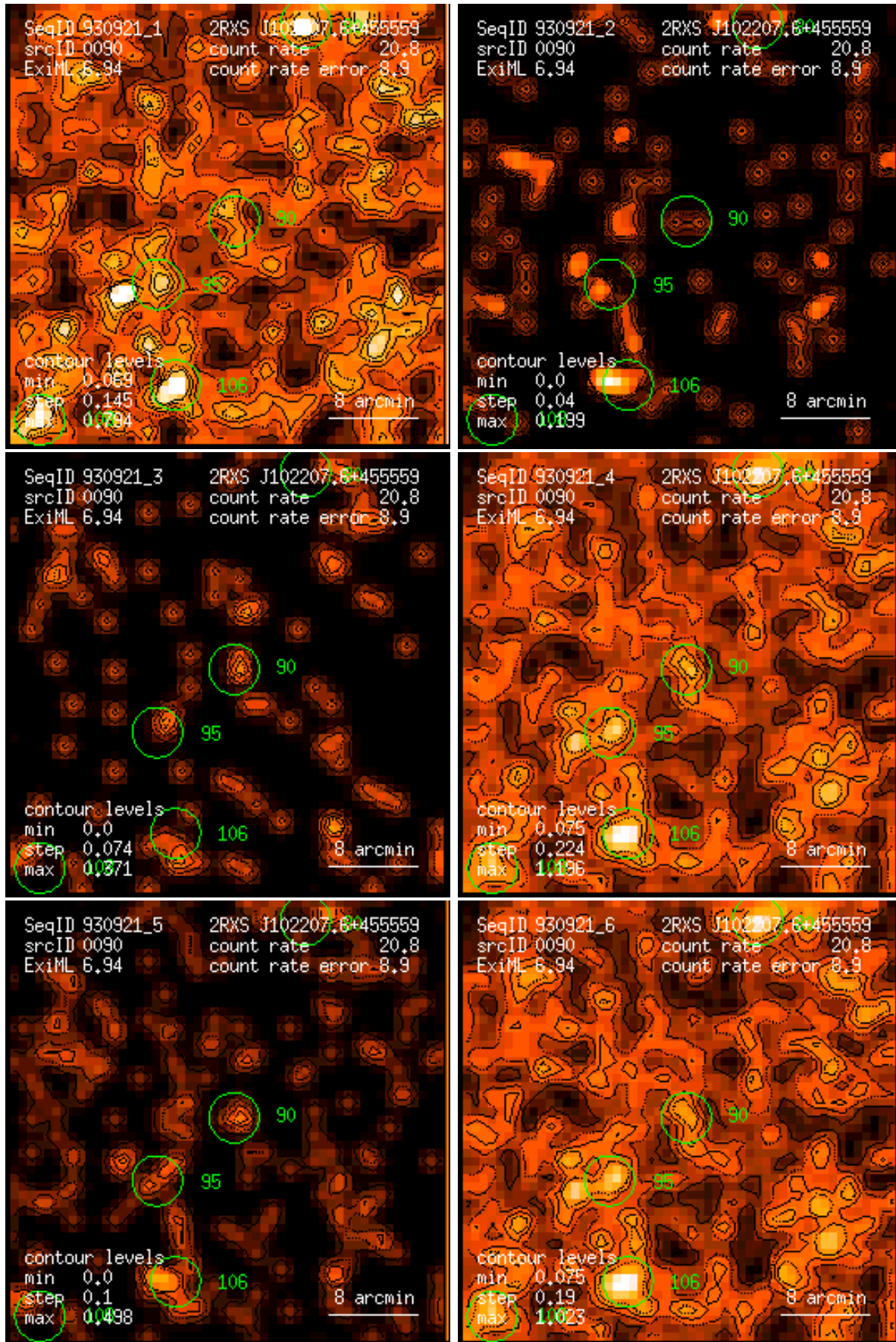
Figure 90: RASS 930921: detection 0090: band rate images, Gaussian filter: (1) PSPC channels 11 – 41, (2) 52 – 90, (3) 91 – 201, (4) 11 – 235, (5) 52 – 201, (6) 11 – 201. Broad band rates in counts/ks. Band rate contour levels in counts/ks/arcmin 2 .
