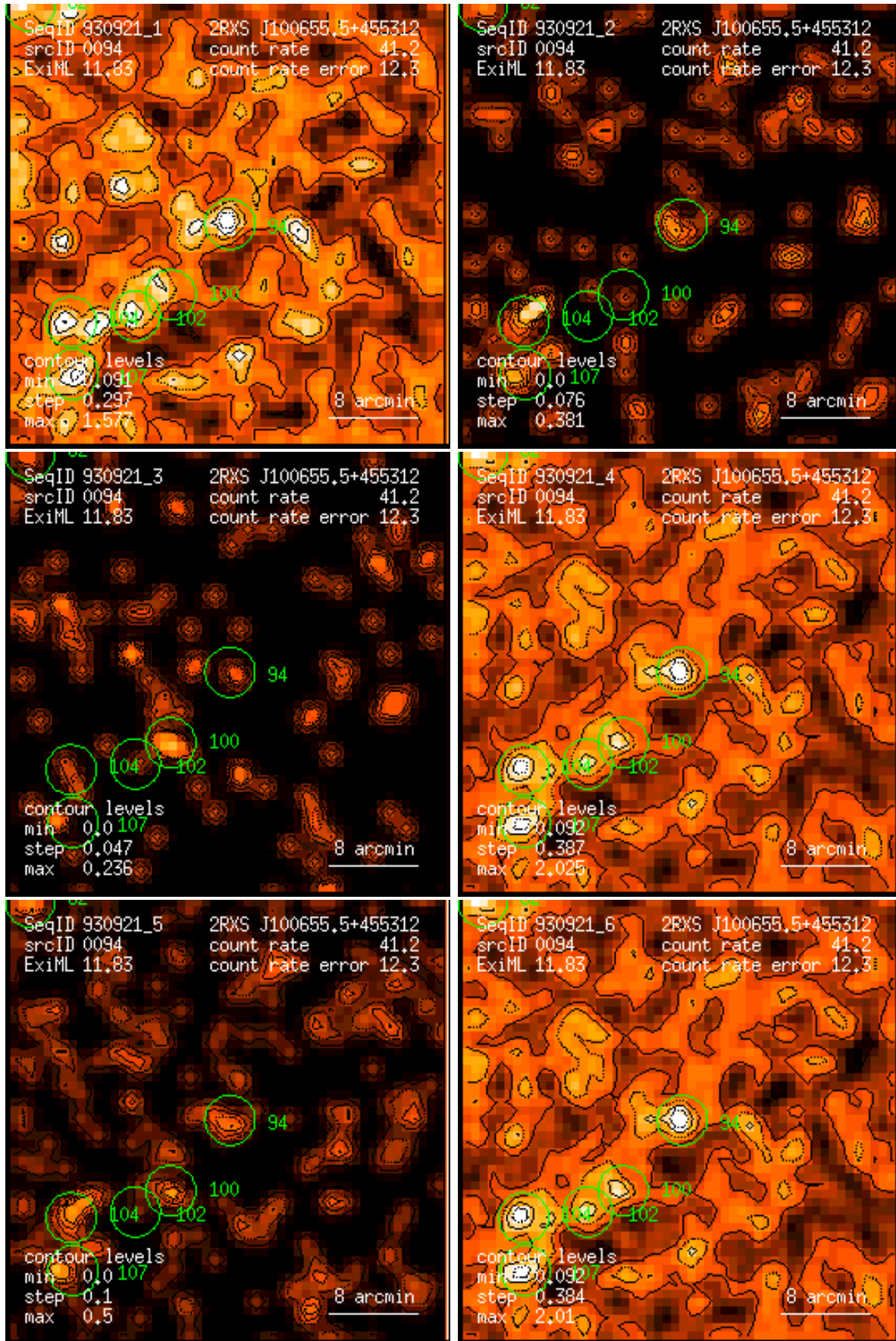
Figure 94: RASS 930921: detection 0094: band rate images, Gaussian filter: (1) PSPC channels 11 – 41, (2) 52 – 90, (3) 91 – 201, (4) 11 – 235, (5) 52 – 201, (6) 11 – 201. Broad band rates in counts/ks. Band rate contour levels in counts/ks/arcmin 2 .
