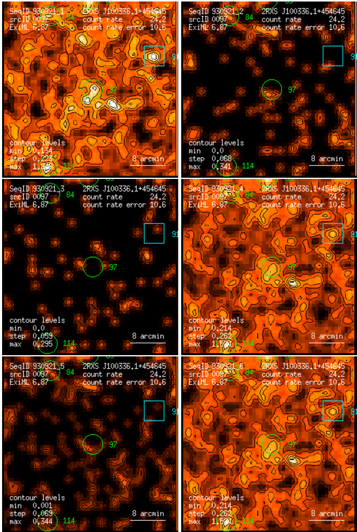
Figure 97: RASS 930921: detection 0097: band rate images, Gaussian filter: (1) PSPC channels 11 – 41, (2) 52 – 90, (3) 91 – 201, (4) 11 – 235, (5) 52 – 201, (6) 11 – 201. Broad band rates in counts/ks. Band rate contour levels in counts/ks/arcmin 2 .
