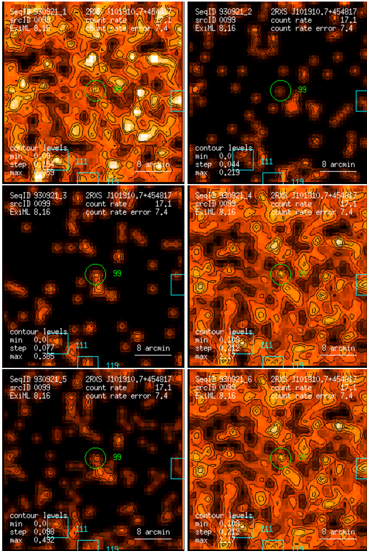
Figure 99: RASS 930921: detection 0099: band rate images, Gaussian filter: (1) PSPC channels 11 – 41, (2) 52 – 90, (3) 91 – 201, (4) 11 – 235, (5) 52 – 201, (6) 11 – 201. Broad band rates in counts/ks. Band rate contour levels in counts/ks/arcmin 2 .
