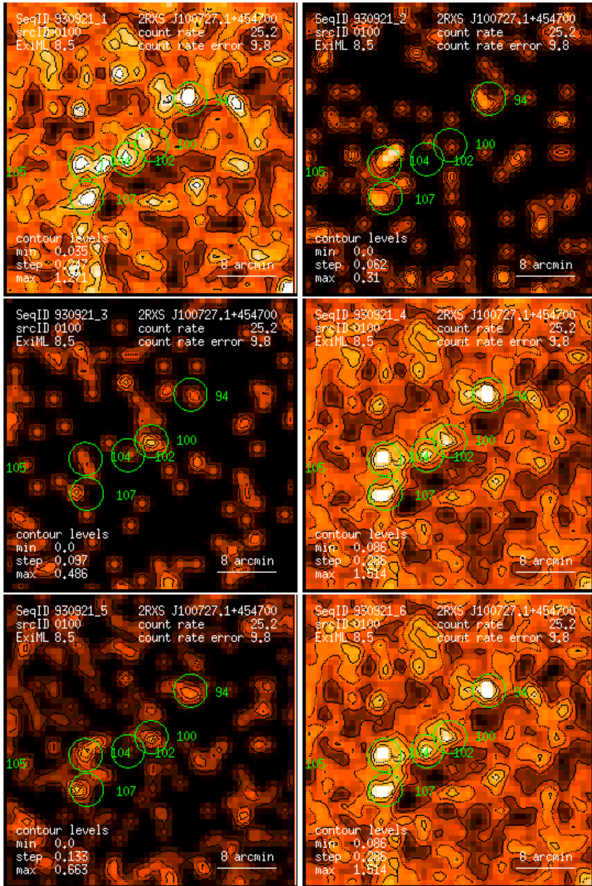
Figure 100: RASS 930921: detection 0100: band rate images, Gaussian filter: (1) PSPC channels 11 – 41, (2) 52 – 90, (3) 91 – 201, (4) 11 – 235, (5) 52 – 201, (6) 11 – 201. Broad band rates in counts/ks. Band rate contour levels in counts/ks/arcmin 2 .
