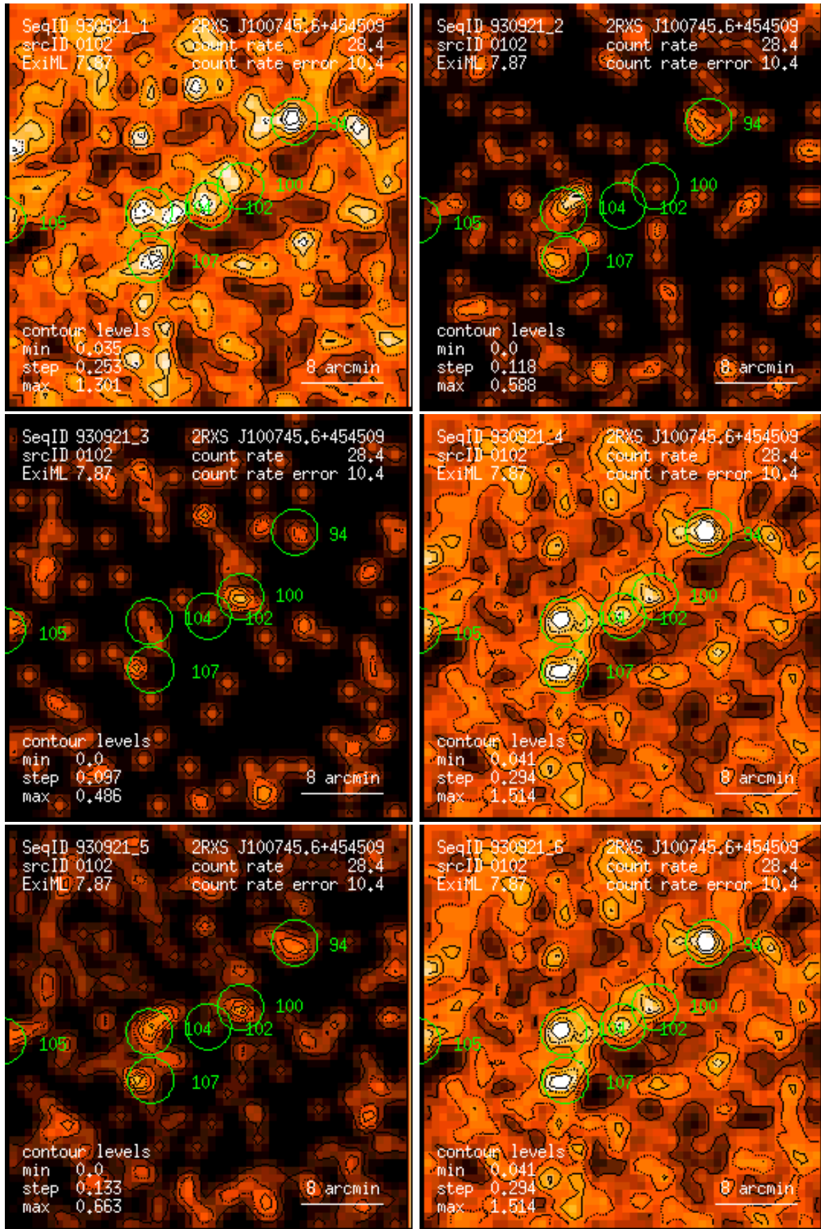
Figure 102: RASS 930921: detection 0102: band rate images, Gaussian filter: (1) PSPC channels 11 – 41, (2) 52 – 90, (3) 91 – 201, (4) 11 – 235, (5) 52 – 201, (6) 11 – 201. Broad band rates in counts/ks. Band rate contour levels in counts/ks/arcmin 2 .
