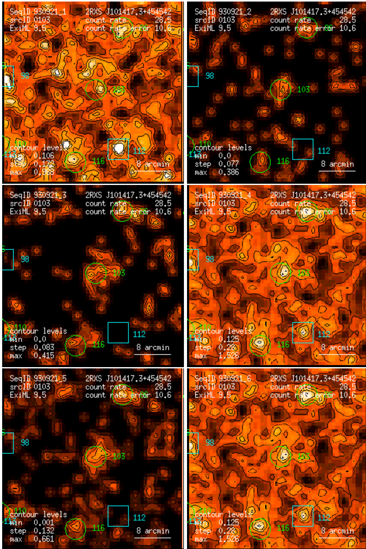
Figure 103: RASS 930921: detection 0103: band rate images, Gaussian filter: (1) PSPC channels 11 – 41, (2) 52 – 90, (3) 91 – 201, (4) 11 – 235, (5) 52 – 201, (6) 11 – 201. Broad band rates in counts/ks. Band rate contour levels in counts/ks/arcmin 2 .
