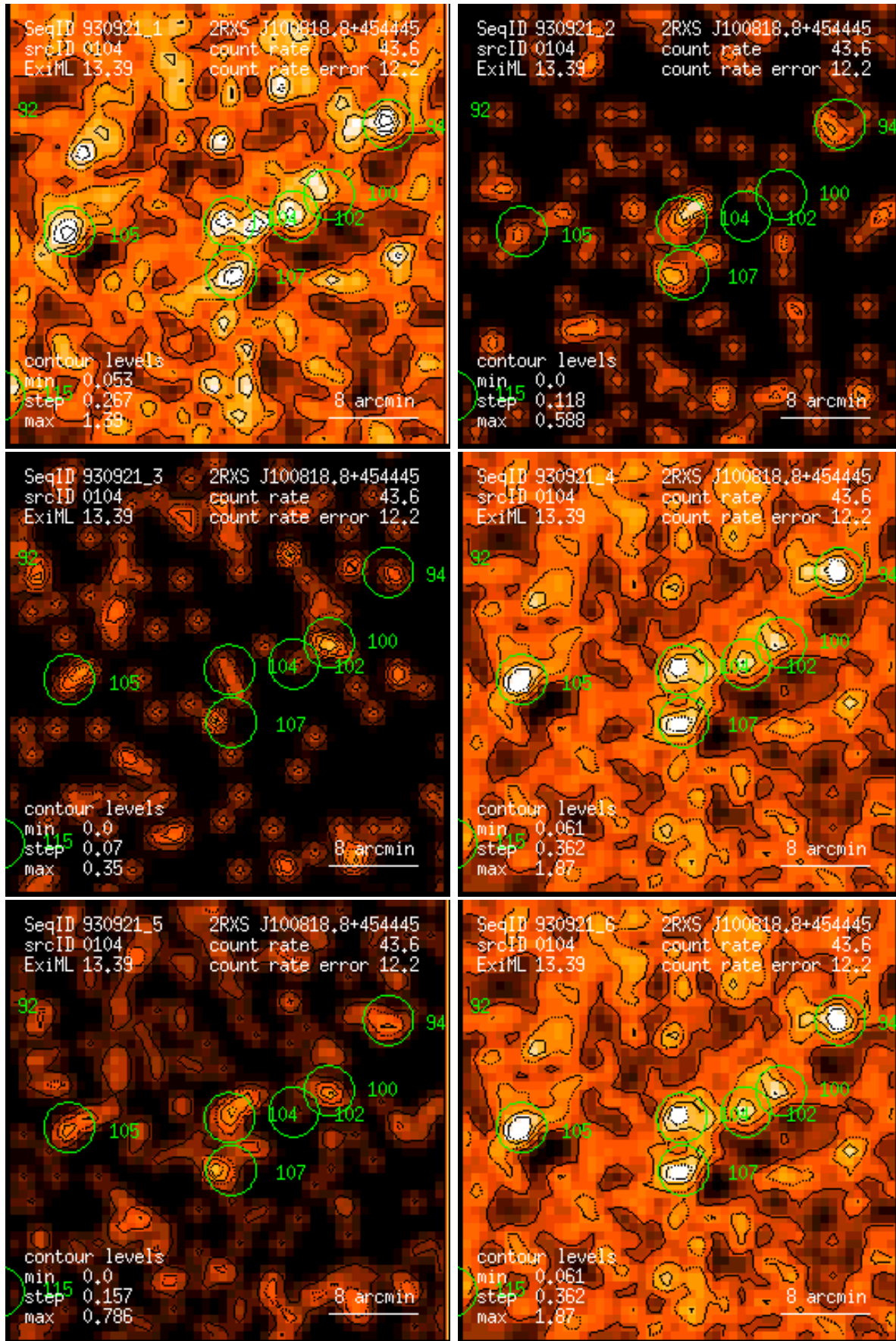
Figure 104: RASS 930921: detection 0104: band rate images, Gaussian filter: (1) PSPC channels 11 – 41, (2) 52 – 90, (3) 91 – 201, (4) 11 – 235, (5) 52 – 201, (6) 11 – 201. Broad band rates in counts/ks. Band rate contour levels in counts/ks/arcmin 2 .
