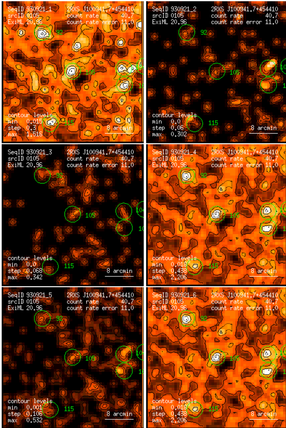
Figure 105: RASS 930921: detection 0105: band rate images, Gaussian filter: (1) PSPC channels 11 – 41, (2) 52 – 90, (3) 91 – 201, (4) 11 – 235, (5) 52 – 201, (6) 11 – 201. Broad band rates in counts/ks. Band rate contour levels in counts/ks/arcmin 2 .
