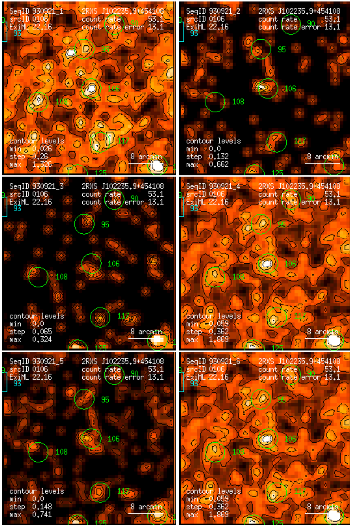
Figure 106: RASS 930921: detection 0106: band rate images, Gaussian filter: (1) PSPC channels 11 – 41, (2) 52 – 90, (3) 91 – 201, (4) 11 – 235, (5) 52 – 201, (6) 11 – 201. Broad band rates in counts/ks. Band rate contour levels in counts/ks/arcmin 2 .
