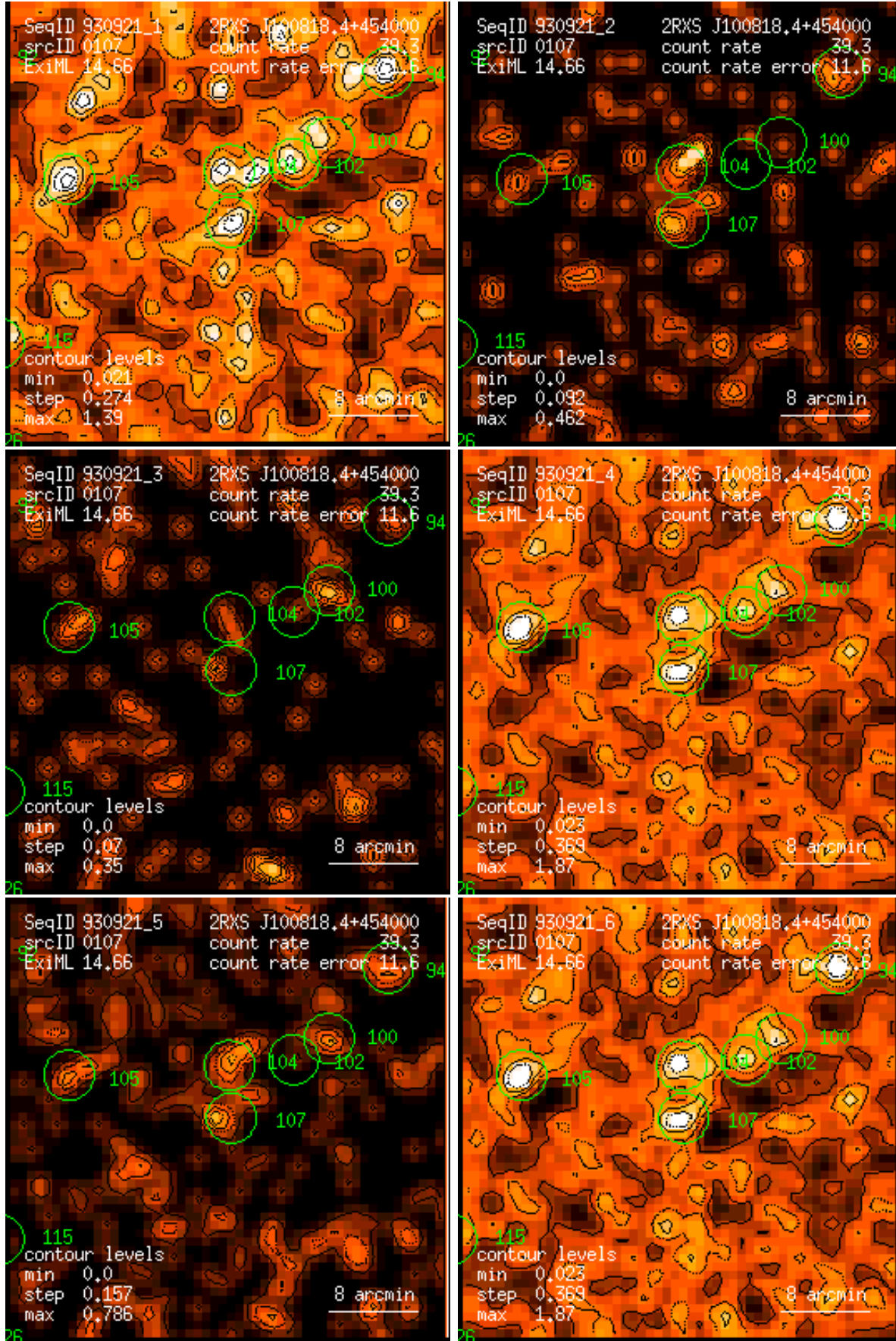
Figure 107: RASS 930921: detection 0107: band rate images, Gaussian filter: (1) PSPC channels 11 – 41, (2) 52 – 90, (3) 91 – 201, (4) 11 – 235, (5) 52 – 201, (6) 11 – 201. Broad band rates in counts/ks. Band rate contour levels in counts/ks/arcmin 2 .
