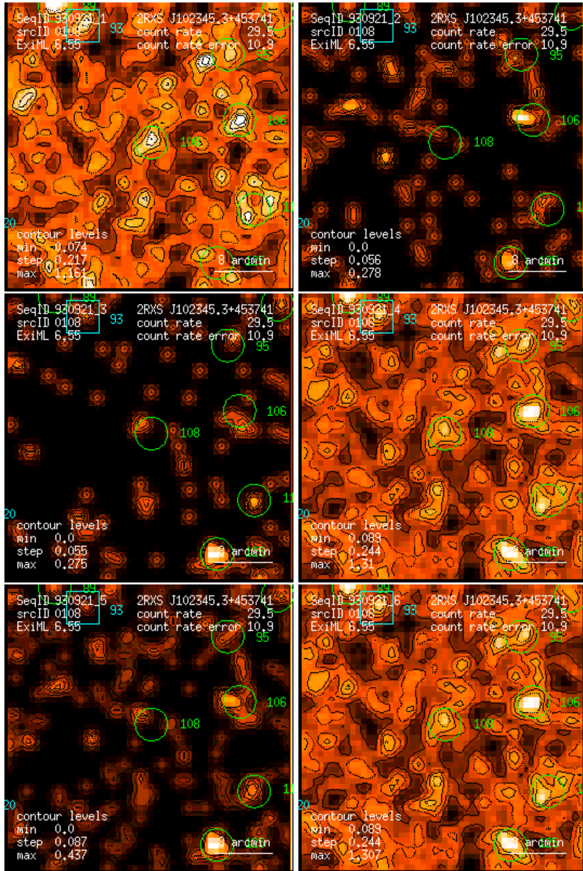
Figure 108: RASS 930921: detection 0108: band rate images, Gaussian filter: (1) PSPC channels 11 – 41, (2) 52 – 90, (3) 91 – 201, (4) 11 – 235, (5) 52 – 201, (6) 11 – 201. Broad band rates in counts/ks. Band rate contour levels in counts/ks/arcmin 2 .
