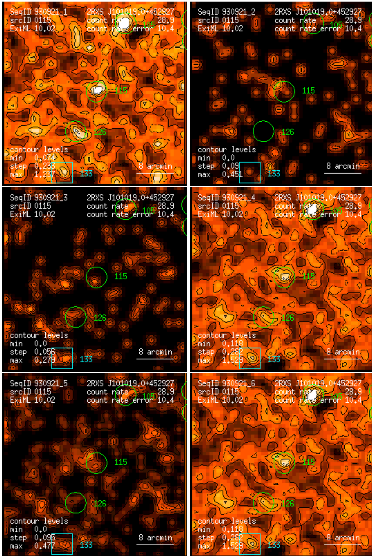
Figure 115: RASS 930921: detection 0115: band rate images, Gaussian filter: (1) PSPC channels 11 – 41, (2) 52 – 90, (3) 91 – 201, (4) 11 – 235, (5) 52 – 201, (6) 11 – 201. Broad band rates in counts/ks. Band rate contour levels in counts/ks/arcmin 2 .
