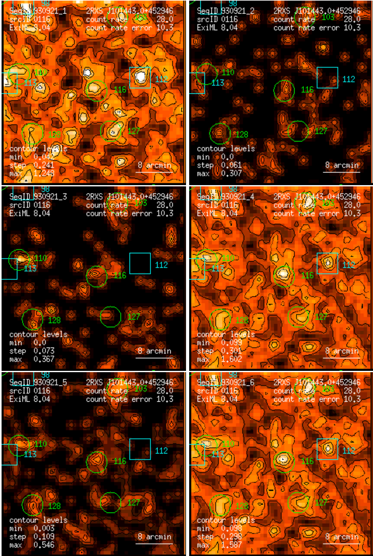
Figure 116: RASS 930921: detection 0116: band rate images, Gaussian filter: (1) PSPC channels 11 – 41, (2) 52 – 90, (3) 91 – 201, (4) 11 – 235, (5) 52 – 201, (6) 11 – 201. Broad band rates in counts/ks. Band rate contour levels in counts/ks/arcmin 2 .
