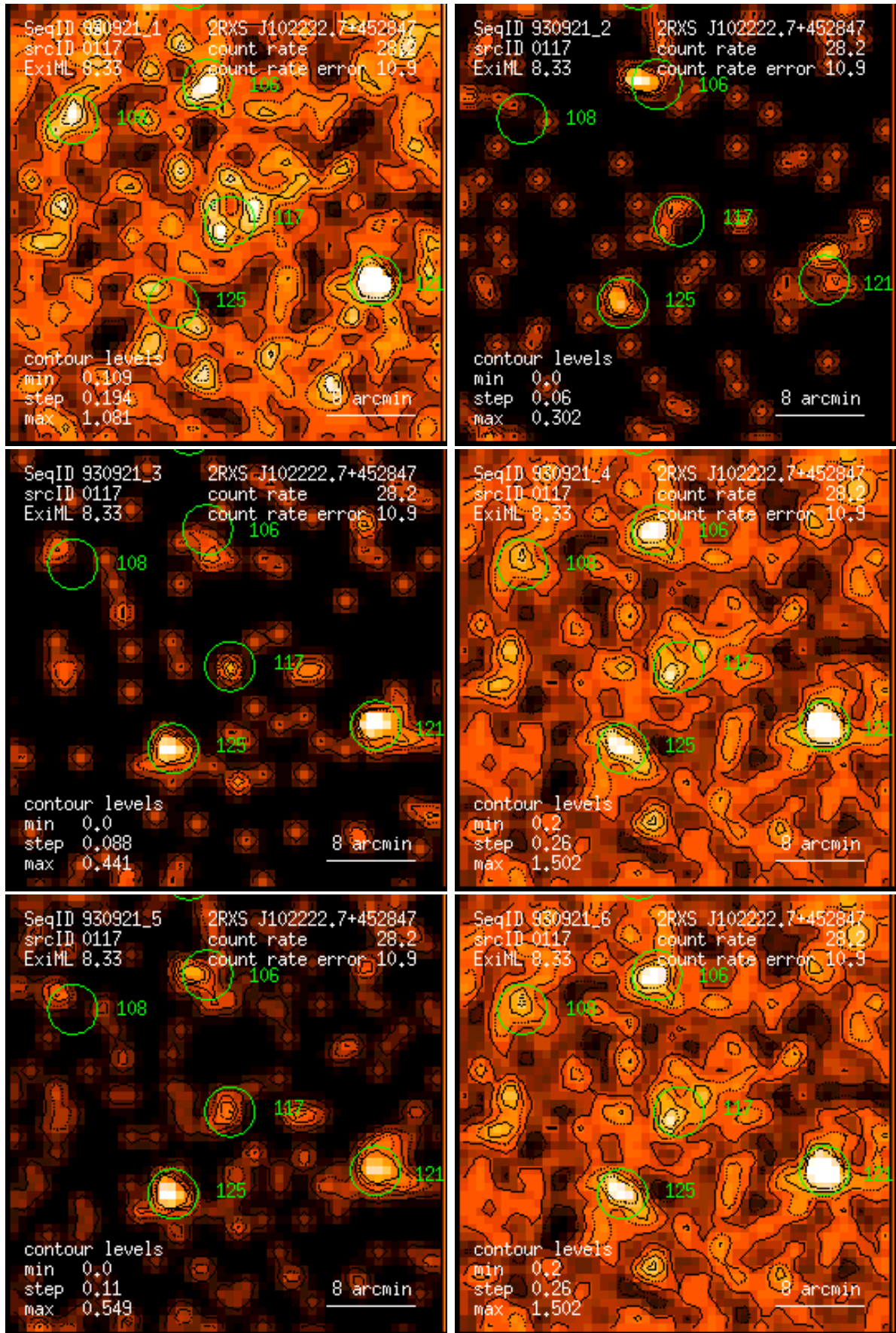
Figure 117: RASS 930921: detection 0117: band rate images, Gaussian filter: (1) PSPC channels 11 – 41, (2) 52 – 90, (3) 91 – 201, (4) 11 – 235, (5) 52 – 201, (6) 11 – 201. Broad band rates in counts/ks. Band rate contour levels in counts/ks/arcmin 2 .
