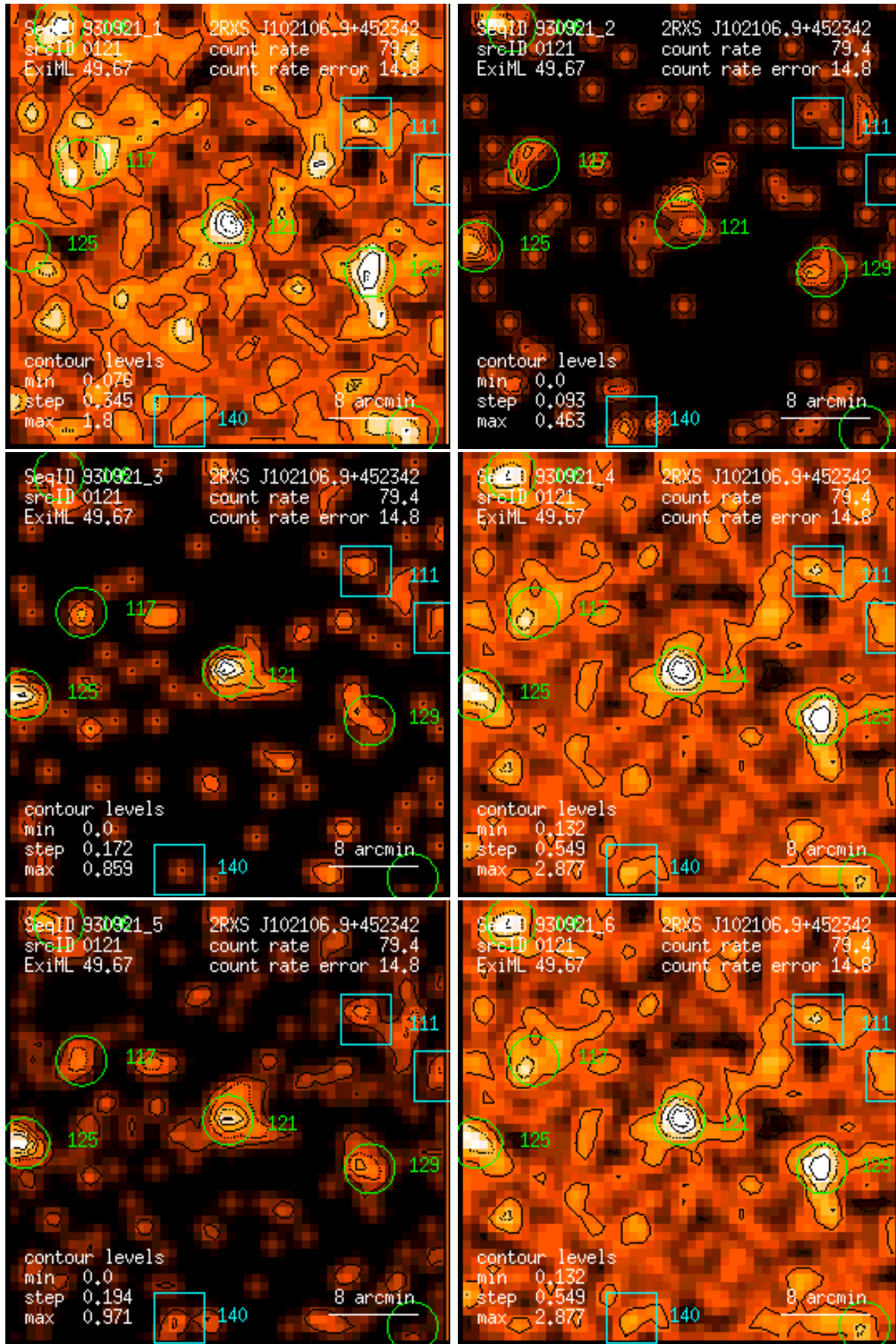
Figure 121: RASS 930921: detection 0121: band rate images, Gaussian filter: (1) PSPC channels 11 – 41, (2) 52 – 90, (3) 91 – 201, (4) 11 – 235, (5) 52 – 201, (6) 11 – 201. Broad band rates in counts/ks. Band rate contour levels in counts/ks/arcmin 2 .
