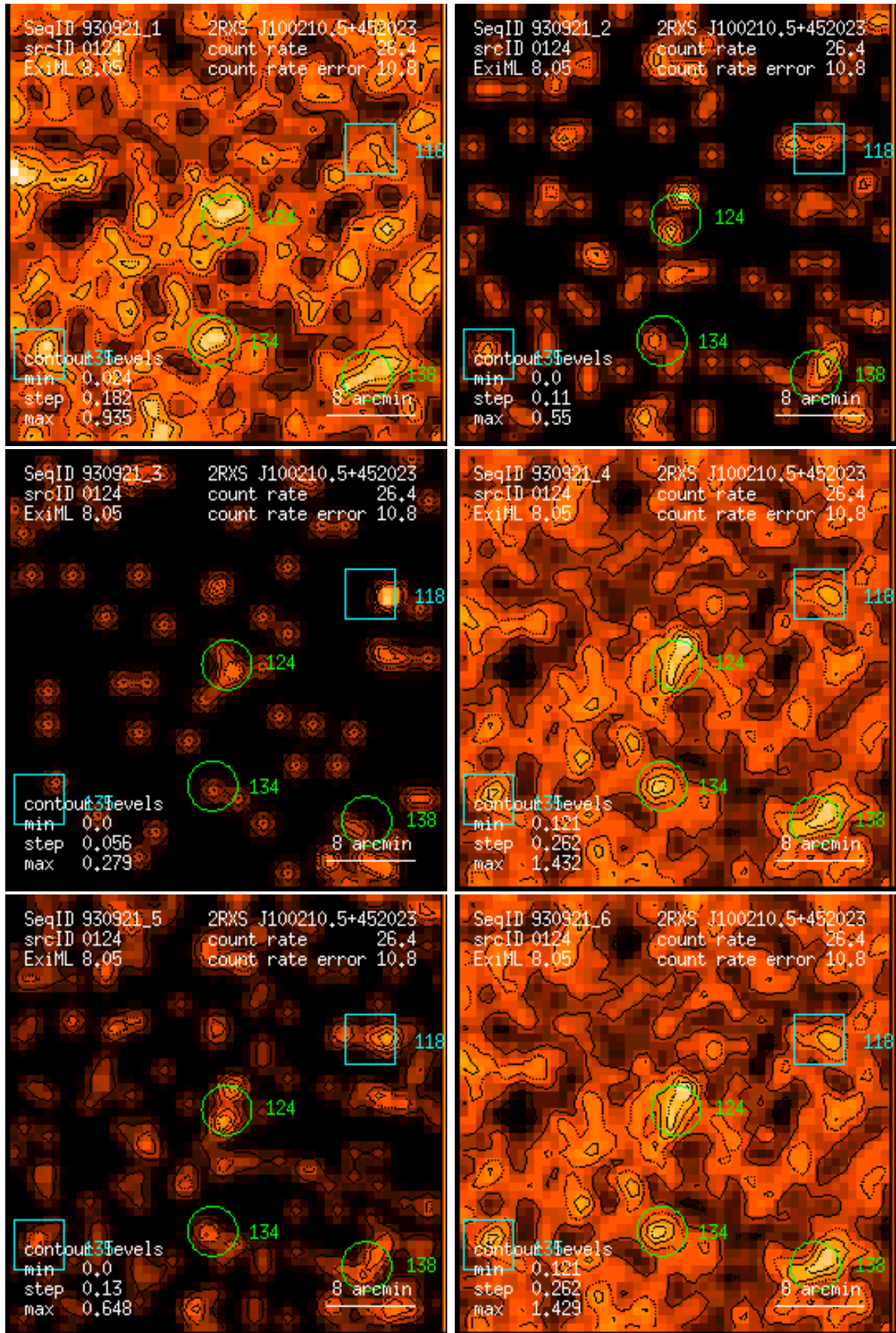
Figure 124: RASS 930921: detection 0124: band rate images, Gaussian filter: (1) PSPC channels 11 – 41, (2) 52 – 90, (3) 91 – 201, (4) 11 – 235, (5) 52 – 201, (6) 11 – 201. Broad band rates in counts/ks. Band rate contour levels in counts/ks/arcmin 2 .
