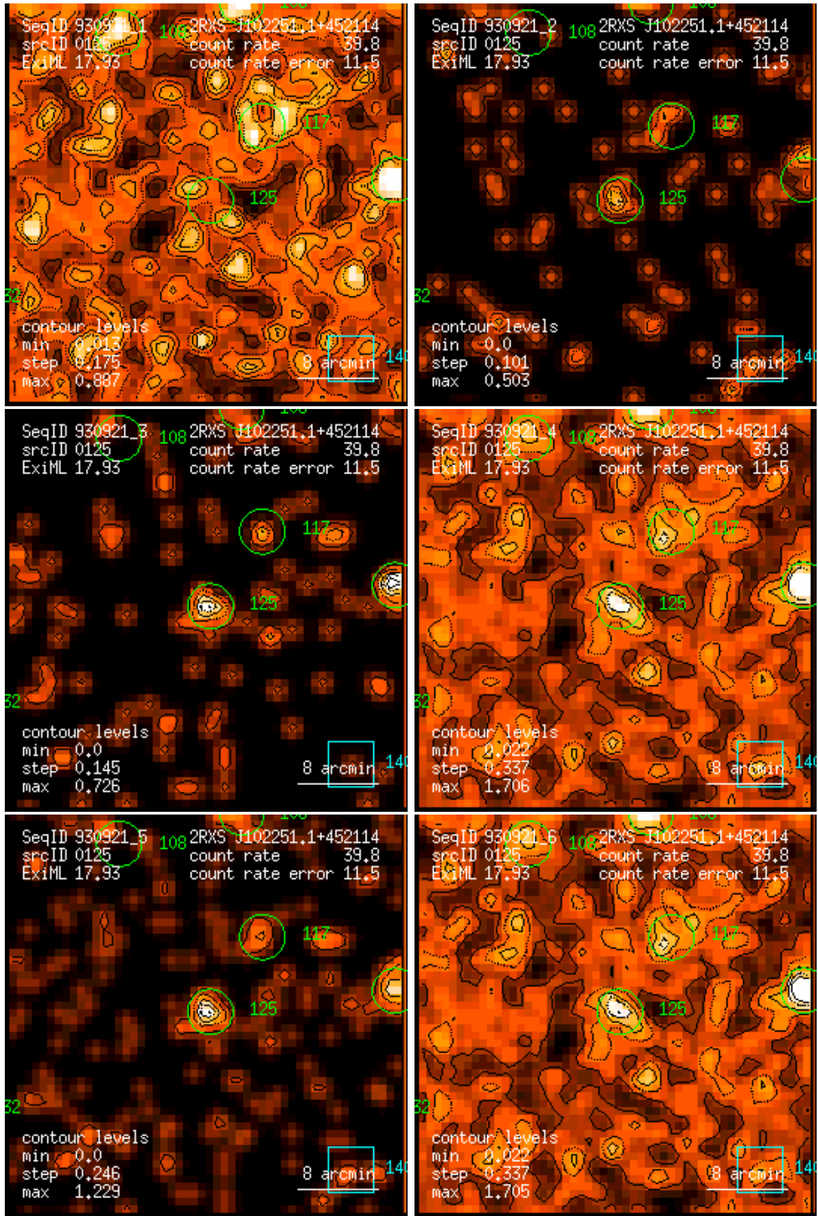
Figure 125: RASS 930921: detection 0125: band rate images, Gaussian filter: (1) PSPC channels 11 – 41, (2) 52 – 90, (3) 91 – 201, (4) 11 – 235, (5) 52 – 201, (6) 11 – 201. Broad band rates in counts/ks. Band rate contour levels in counts/ks/arcmin 2 .
