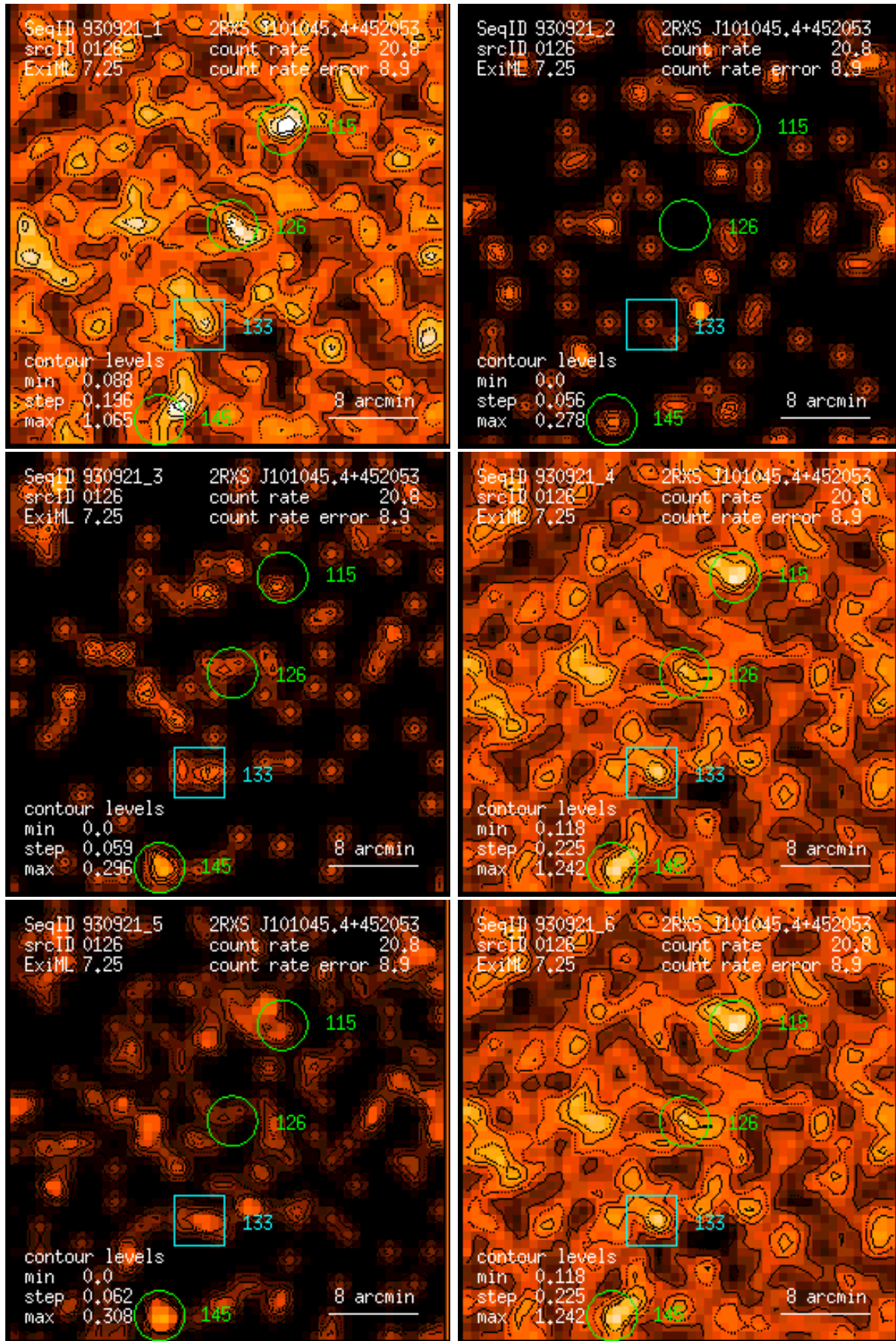
Figure 126: RASS 930921: detection 0126: band rate images, Gaussian filter: (1) PSPC channels 11 – 41, (2) 52 – 90, (3) 91 – 201, (4) 11 – 235, (5) 52 – 201, (6) 11 – 201. Broad band rates in counts/ks. Band rate contour levels in counts/ks/arcmin 2 .
