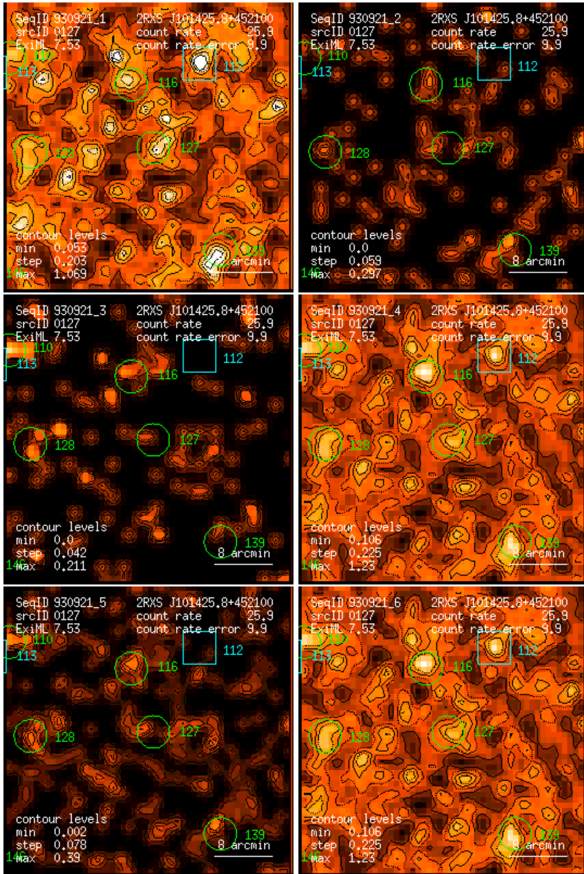
Figure 127: RASS 930921: detection 0127: band rate images, Gaussian filter: (1) PSPC channels 11 – 41, (2) 52 – 90, (3) 91 – 201, (4) 11 – 235, (5) 52 – 201, (6) 11 – 201. Broad band rates in counts/ks. Band rate contour levels in counts/ks/arcmin 2 .
