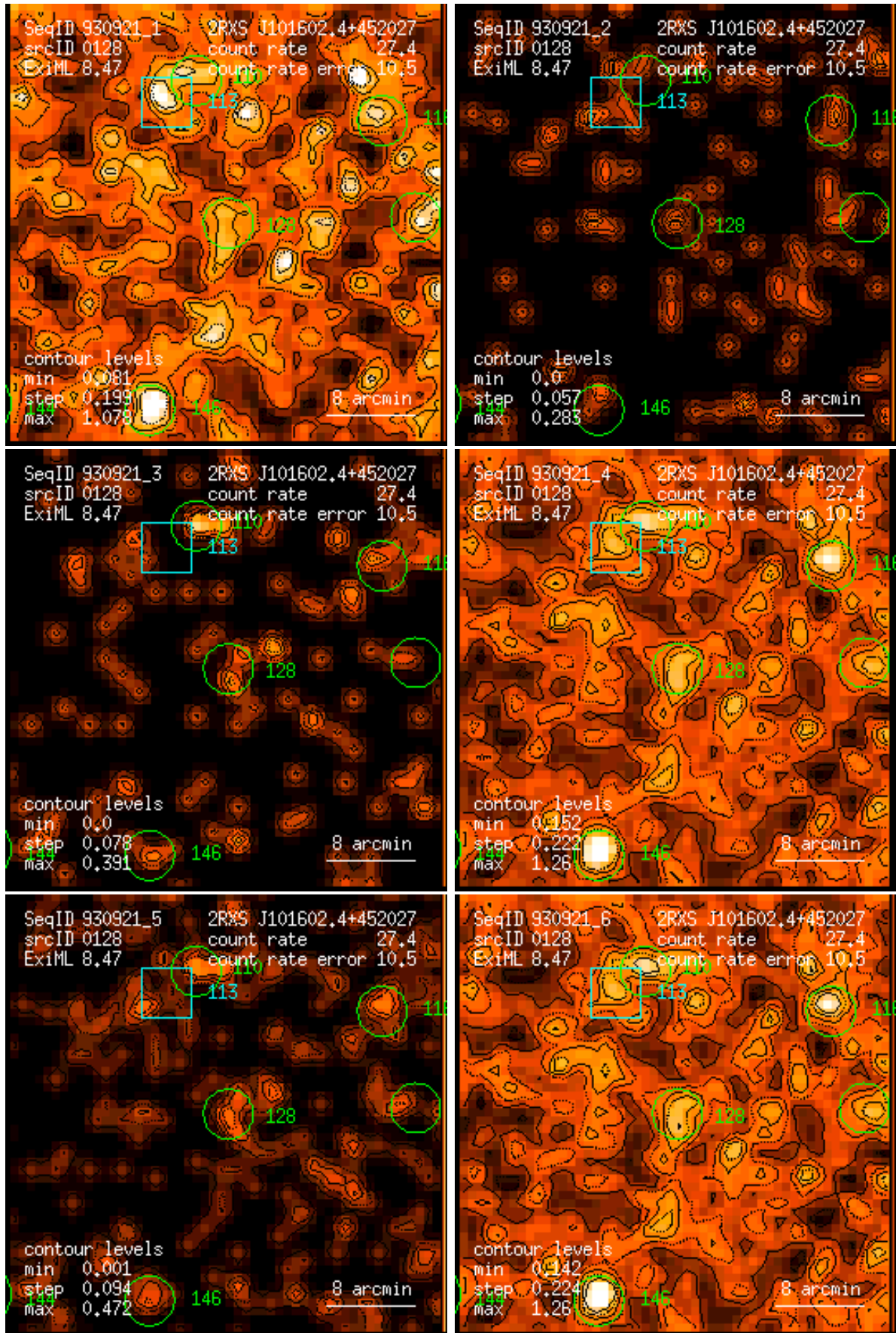
Figure 128: RASS 930921: detection 0128: band rate images, Gaussian filter: (1) PSPC channels 11 – 41, (2) 52 – 90, (3) 91 – 201, (4) 11 – 235, (5) 52 – 201, (6) 11 – 201. Broad band rates in counts/ks. Band rate contour levels in counts/ks/arcmin 2 .
