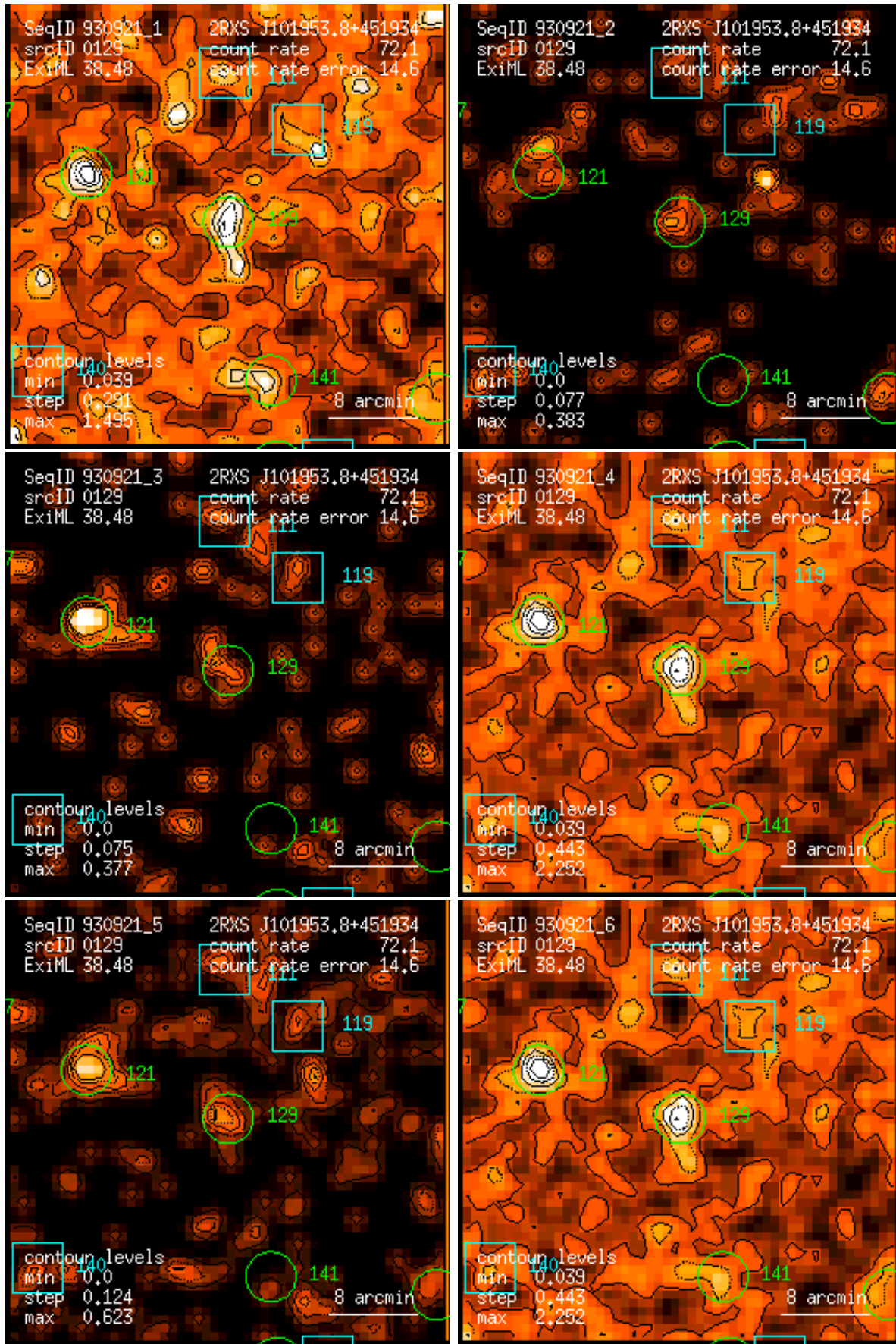
Figure 129: RASS 930921: detection 0129: band rate images, Gaussian filter: (1) PSPC channels 11 – 41, (2) 52 – 90, (3) 91 – 201, (4) 11 – 235, (5) 52 – 201, (6) 11 – 201. Broad band rates in counts/ks. Band rate contour levels in counts/ks/arcmin 2 .
