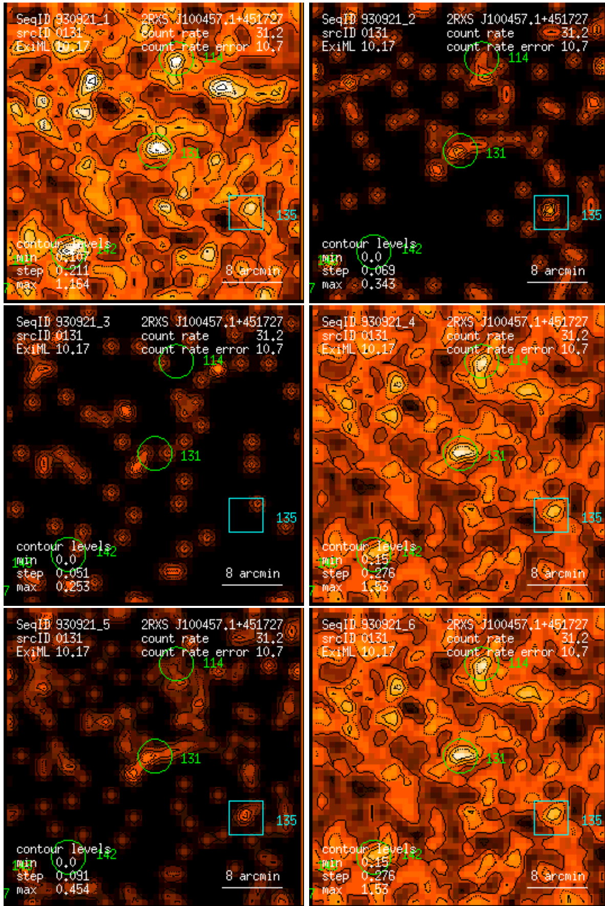
Figure 131: RASS 930921: detection 0131: band rate images, Gaussian filter: (1) PSPC channels 11 – 41, (2) 52 – 90, (3) 91 – 201, (4) 11 – 235, (5) 52 – 201, (6) 11 – 201. Broad band rates in counts/ks. Band rate contour levels in counts/ks/arcmin 2 .
