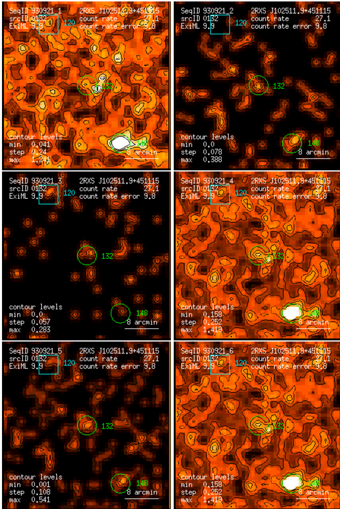
Figure 132: RASS 930921: detection 0132: band rate images, Gaussian filter: (1) PSPC channels 11 – 41, (2) 52 – 90, (3) 91 – 201, (4) 11 – 235, (5) 52 – 201, (6) 11 – 201. Broad band rates in counts/ks. Band rate contour levels in counts/ks/arcmin 2 .
