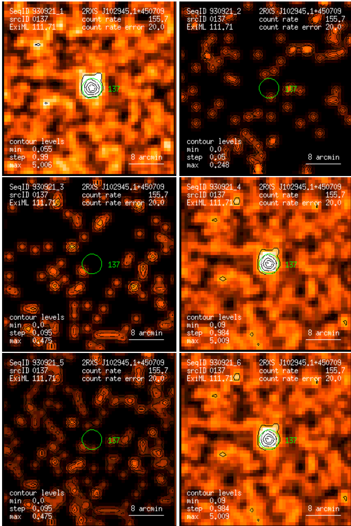
Figure 137: RASS 930921: detection 0137: band rate images, Gaussian filter: (1) PSPC channels 11 – 41, (2) 52 – 90, (3) 91 – 201, (4) 11 – 235, (5) 52 – 201, (6) 11 – 201. Broad band rates in counts/ks. Band rate contour levels in counts/ks/arcmin 2 .
