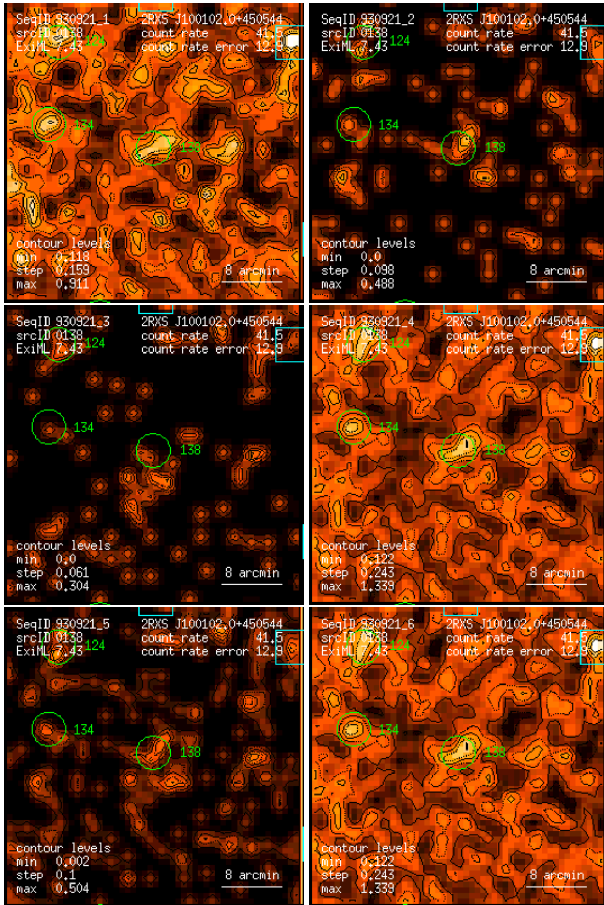
Figure 138: RASS 930921: detection 0138: band rate images, Gaussian filter: (1) PSPC channels 11 – 41, (2) 52 – 90, (3) 91 – 201, (4) 11 – 235, (5) 52 – 201, (6) 11 – 201. Broad band rates in counts/ks. Band rate contour levels in counts/ks/arcmin 2 .
