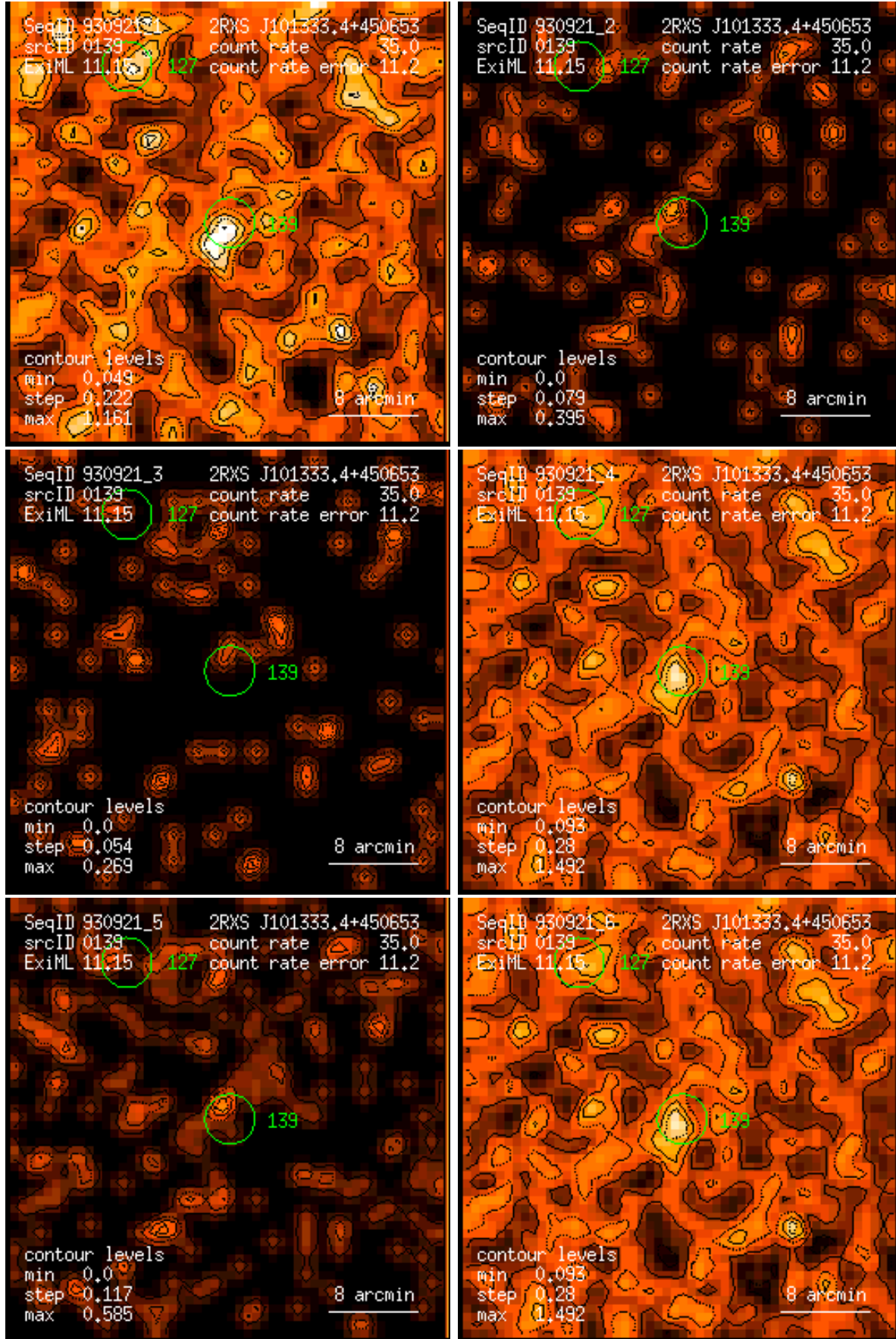
Figure 139: RASS 930921: detection 0139: band rate images, Gaussian filter: (1) PSPC channels 11 – 41, (2) 52 – 90, (3) 91 – 201, (4) 11 – 235, (5) 52 – 201, (6) 11 – 201. Broad band rates in counts/ks. Band rate contour levels in counts/ks/arcmin 2 .
