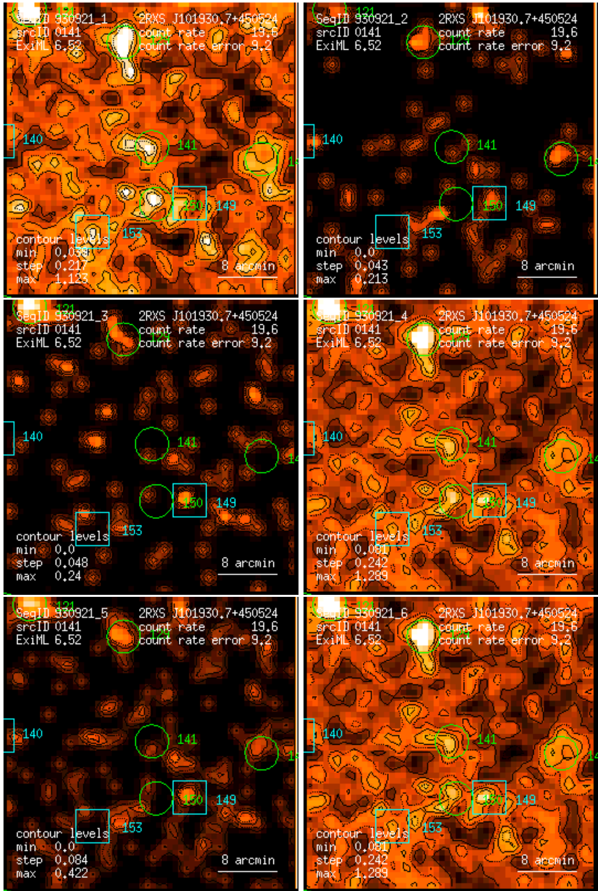
Figure 141: RASS 930921: detection 0141: band rate images, Gaussian filter: (1) PSPC channels 11 – 41, (2) 52 – 90, (3) 91 – 201, (4) 11 – 235, (5) 52 – 201, (6) 11 – 201. Broad band rates in counts/ks. Band rate contour levels in counts/ks/arcmin 2 .
