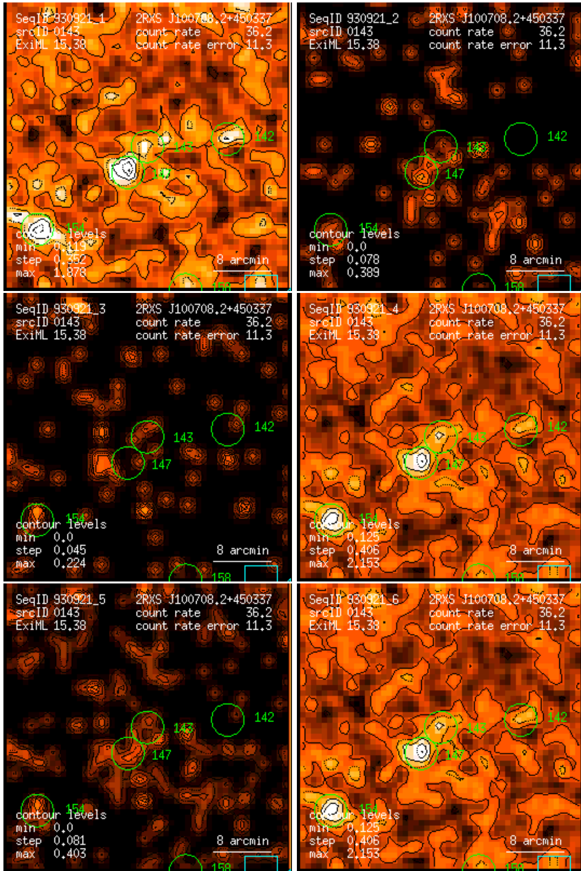
Figure 143: RASS 930921: detection 0143: band rate images, Gaussian filter: (1) PSPC channels 11 – 41, (2) 52 – 90, (3) 91 – 201, (4) 11 – 235, (5) 52 – 201, (6) 11 – 201. Broad band rates in counts/ks. Band rate contour levels in counts/ks/arcmin 2 .
