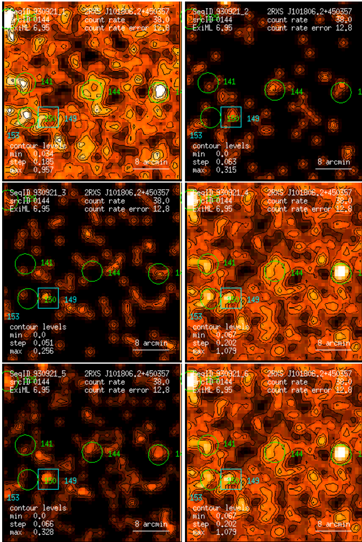
Figure 144: RASS 930921: detection 0144: band rate images, Gaussian filter: (1) PSPC channels 11 – 41, (2) 52 – 90, (3) 91 – 201, (4) 11 – 235, (5) 52 – 201, (6) 11 – 201. Broad band rates in counts/ks. Band rate contour levels in counts/ks/arcmin 2 .
