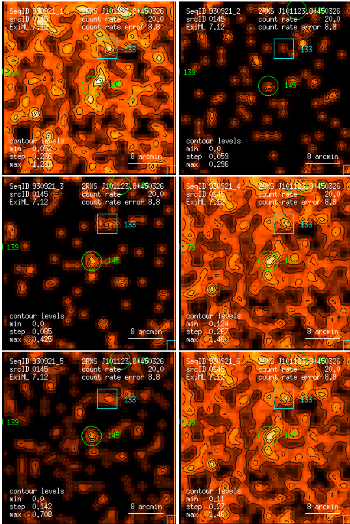
Figure 145: RASS 930921: detection 0145: band rate images, Gaussian filter: (1) PSPC channels 11 – 41, (2) 52 – 90, (3) 91 – 201, (4) 11 – 235, (5) 52 – 201, (6) 11 – 201. Broad band rates in counts/ks. Band rate contour levels in counts/ks/arcmin 2 .
