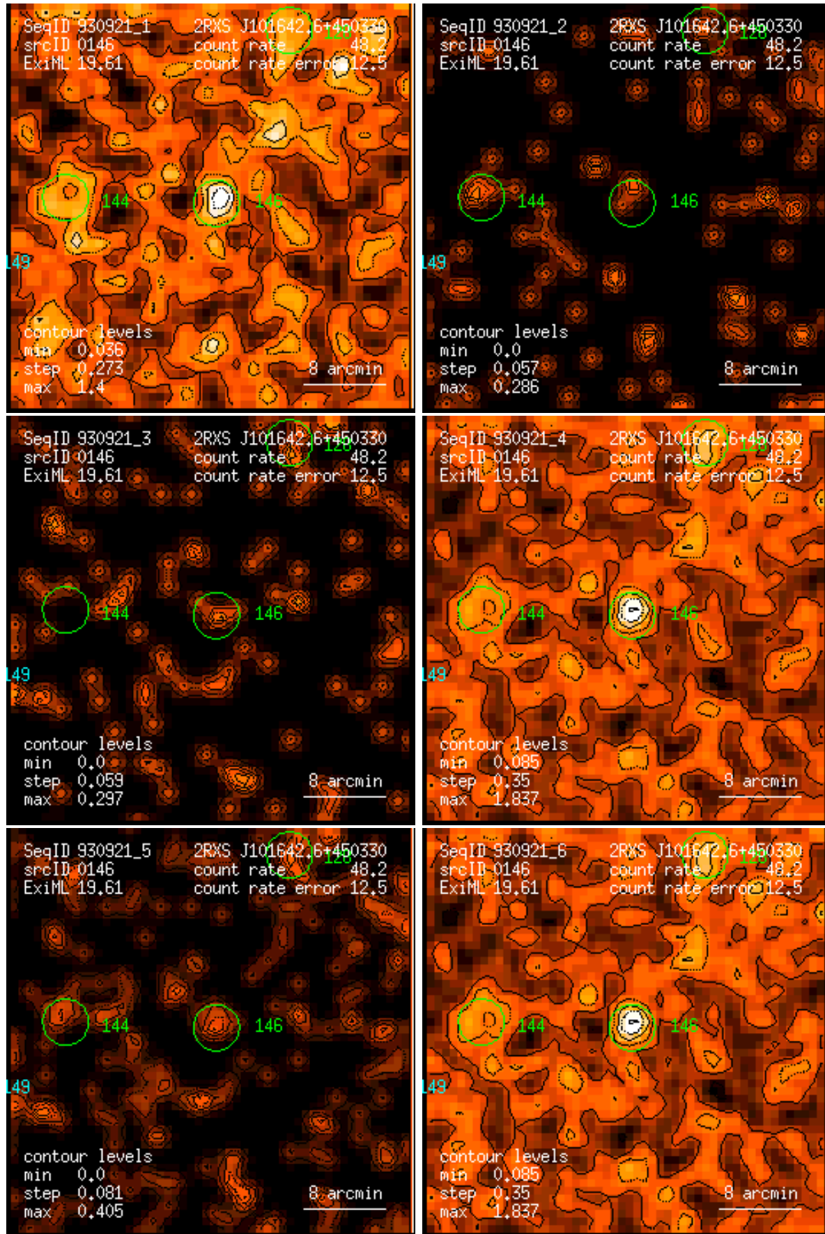
Figure 146: RASS 930921: detection 0146: band rate images, Gaussian filter: (1) PSPC channels 11 – 41, (2) 52 – 90, (3) 91 – 201, (4) 11 – 235, (5) 52 – 201, (6) 11 – 201. Broad band rates in counts/ks. Band rate contour levels in counts/ks/arcmin 2 .
