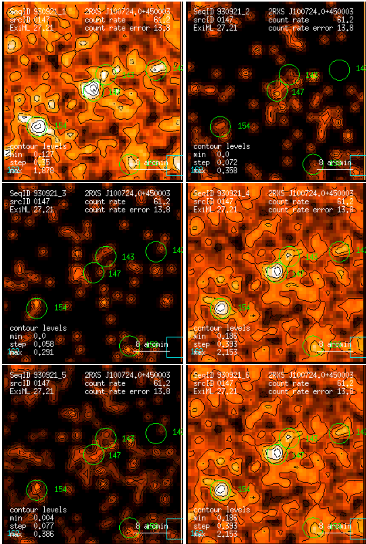
Figure 147: RASS 930921: detection 0147: band rate images, Gaussian filter: (1) PSPC channels 11 – 41, (2) 52 – 90, (3) 91 – 201, (4) 11 – 235, (5) 52 – 201, (6) 11 – 201. Broad band rates in counts/ks. Band rate contour levels in counts/ks/arcmin 2 .
