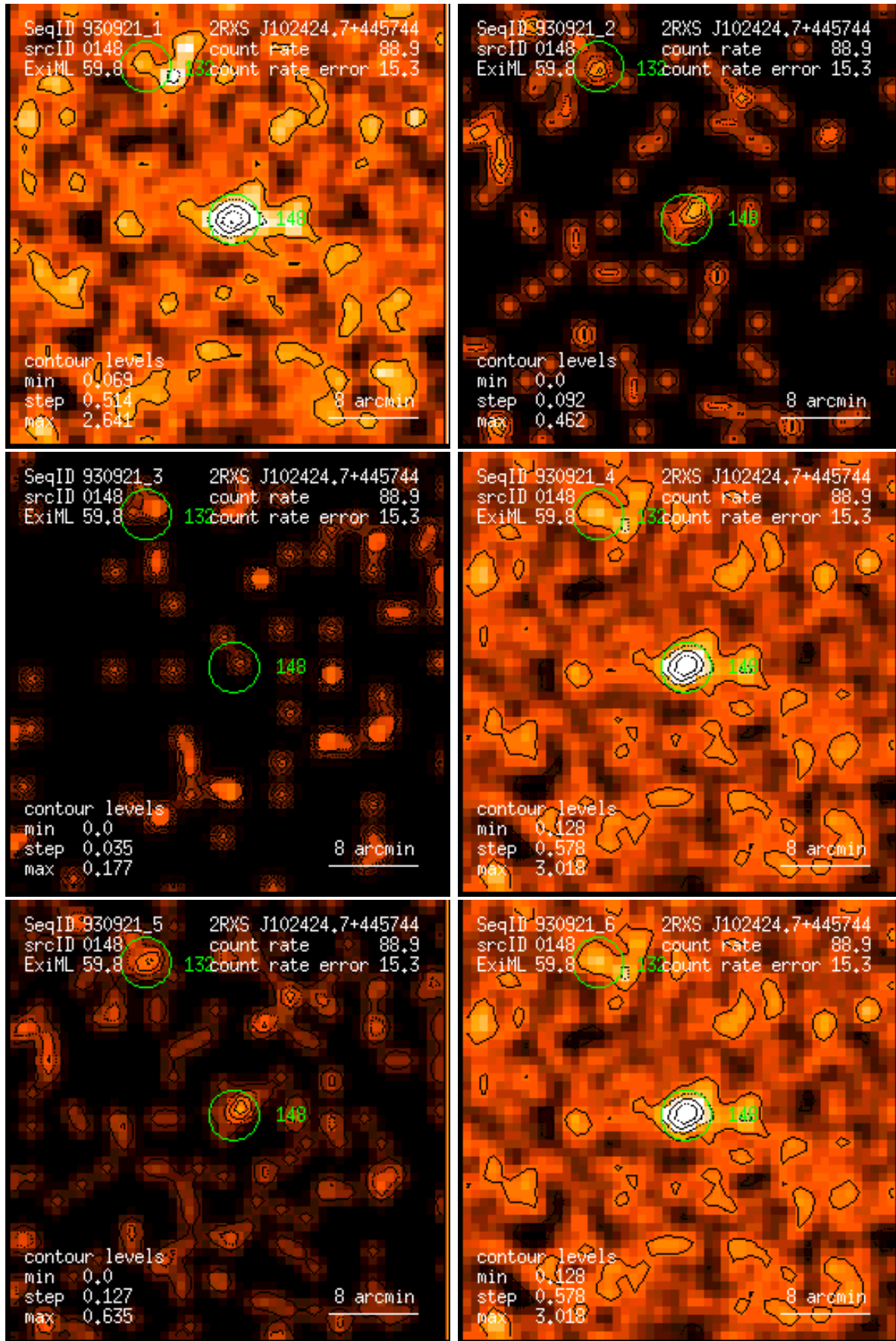
Figure 148: RASS 930921: detection 0148: band rate images, Gaussian filter: (1) PSPC channels 11 – 41, (2) 52 – 90, (3) 91 – 201, (4) 11 – 235, (5) 52 – 201, (6) 11 – 201. Broad band rates in counts/ks. Band rate contour levels in counts/ks/arcmin 2 .
