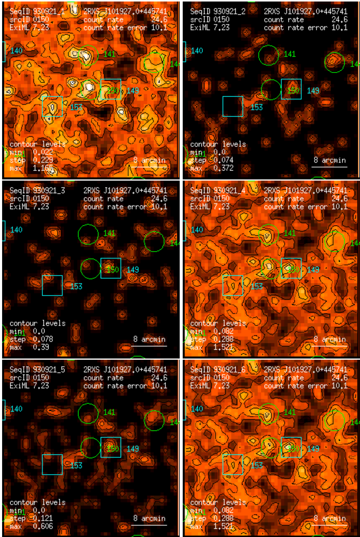
Figure 150: RASS 930921: detection 0150: band rate images, Gaussian filter: (1) PSPC channels 11 – 41, (2) 52 – 90, (3) 91 – 201, (4) 11 – 235, (5) 52 – 201, (6) 11 – 201. Broad band rates in counts/ks. Band rate contour levels in counts/ks/arcmin 2 .
