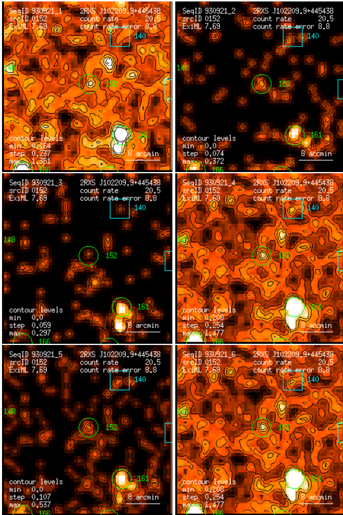
Figure 152: RASS 930921: detection 0152: band rate images, Gaussian filter: (1) PSPC channels 11 – 41, (2) 52 – 90, (3) 91 – 201, (4) 11 – 235, (5) 52 – 201, (6) 11 – 201. Broad band rates in counts/ks. Band rate contour levels in counts/ks/arcmin 2 .
