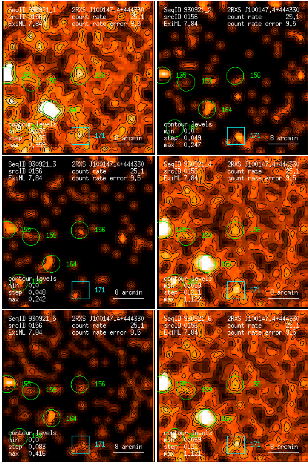
Figure 156: RASS 930921: detection 0156: band rate images, Gaussian filter: (1) PSPC channels 11 – 41, (2) 52 – 90, (3) 91 – 201, (4) 11 – 235, (5) 52 – 201, (6) 11 – 201. Broad band rates in counts/ks. Band rate contour levels in counts/ks/arcmin 2 .
