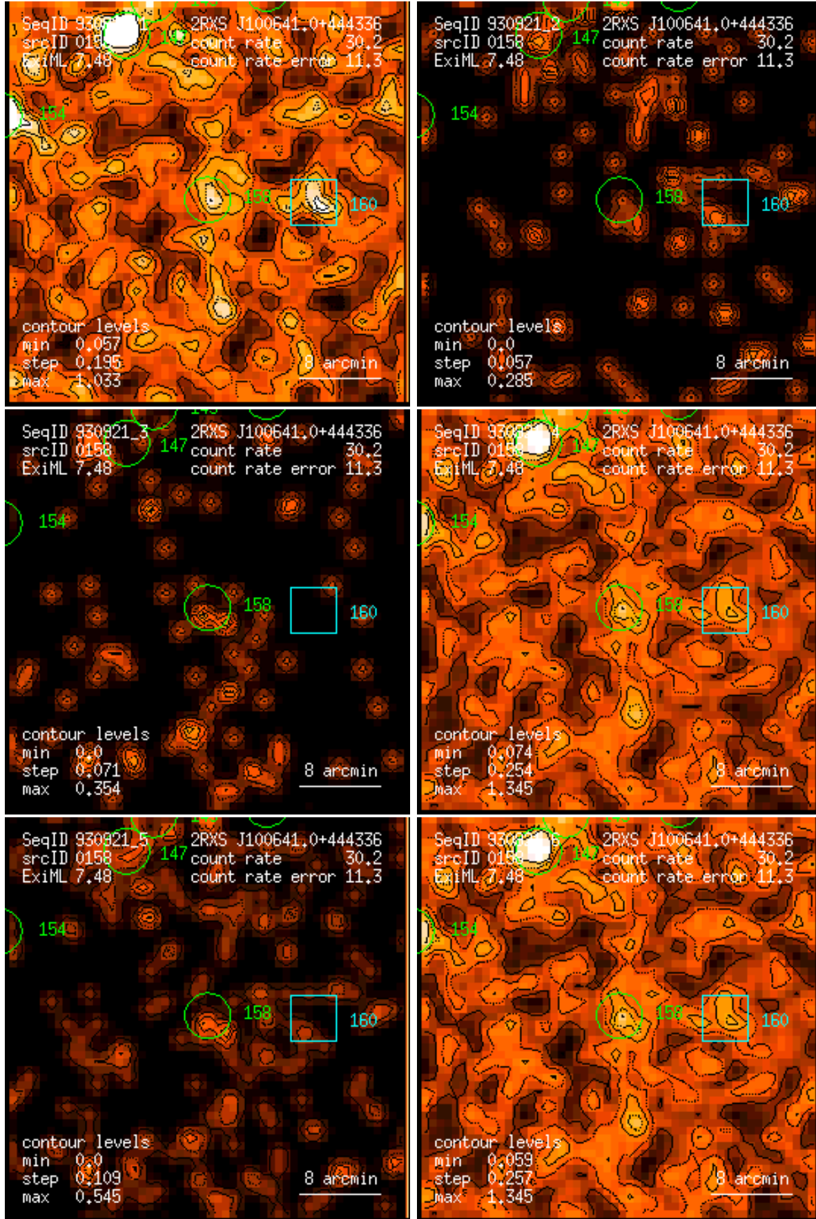
Figure 158: RASS 930921: detection 0158: band rate images, Gaussian filter: (1) PSPC channels 11 – 41, (2) 52 – 90, (3) 91 – 201, (4) 11 – 235, (5) 52 – 201, (6) 11 – 201. Broad band rates in counts/ks. Band rate contour levels in counts/ks/arcmin 2 .
