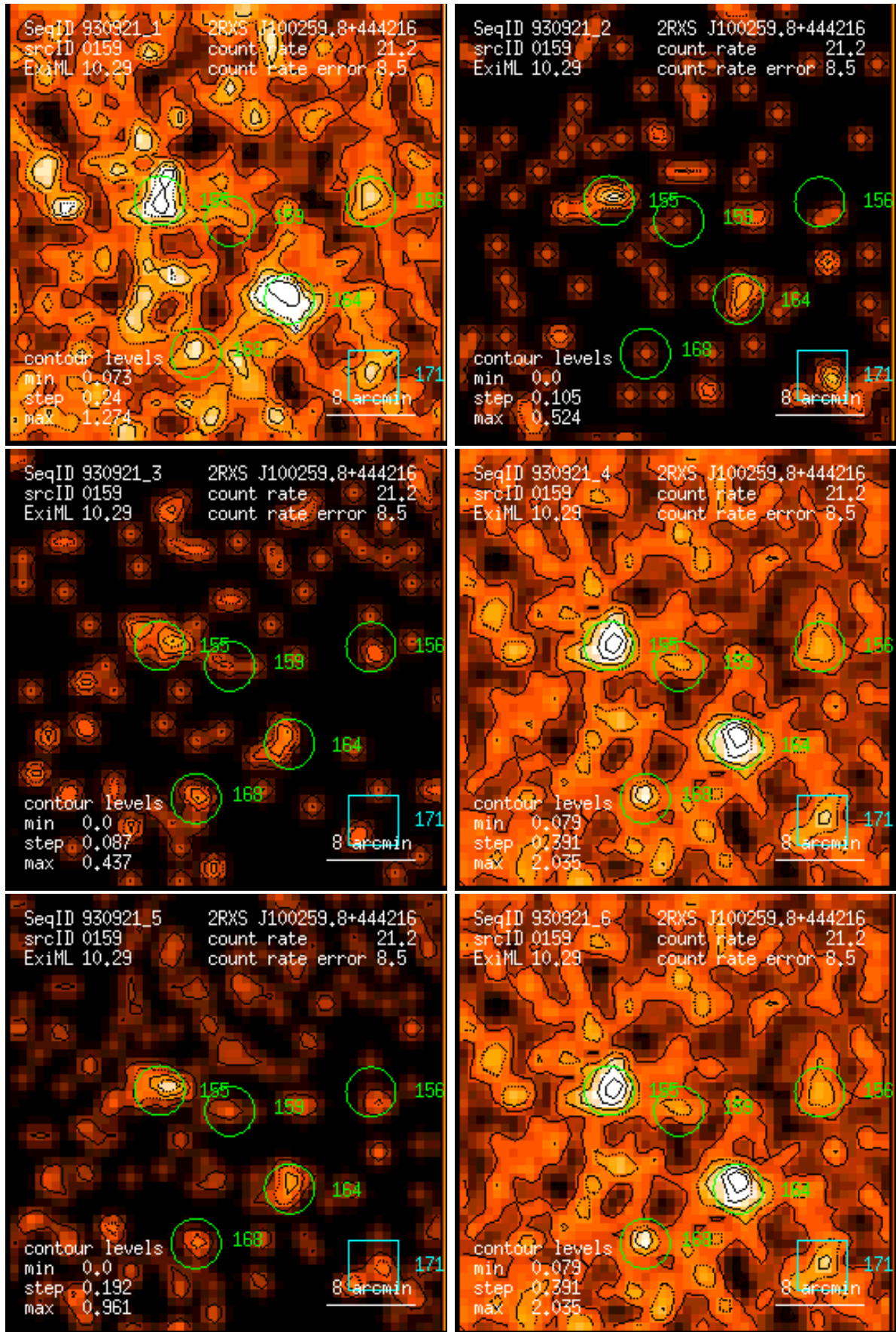
Figure 159: RASS 930921: detection 0159: band rate images, Gaussian filter: (1) PSPC channels 11 – 41, (2) 52 – 90, (3) 91 – 201, (4) 11 – 235, (5) 52 – 201, (6) 11 – 201. Broad band rates in counts/ks. Band rate contour levels in counts/ks/arcmin 2 .
