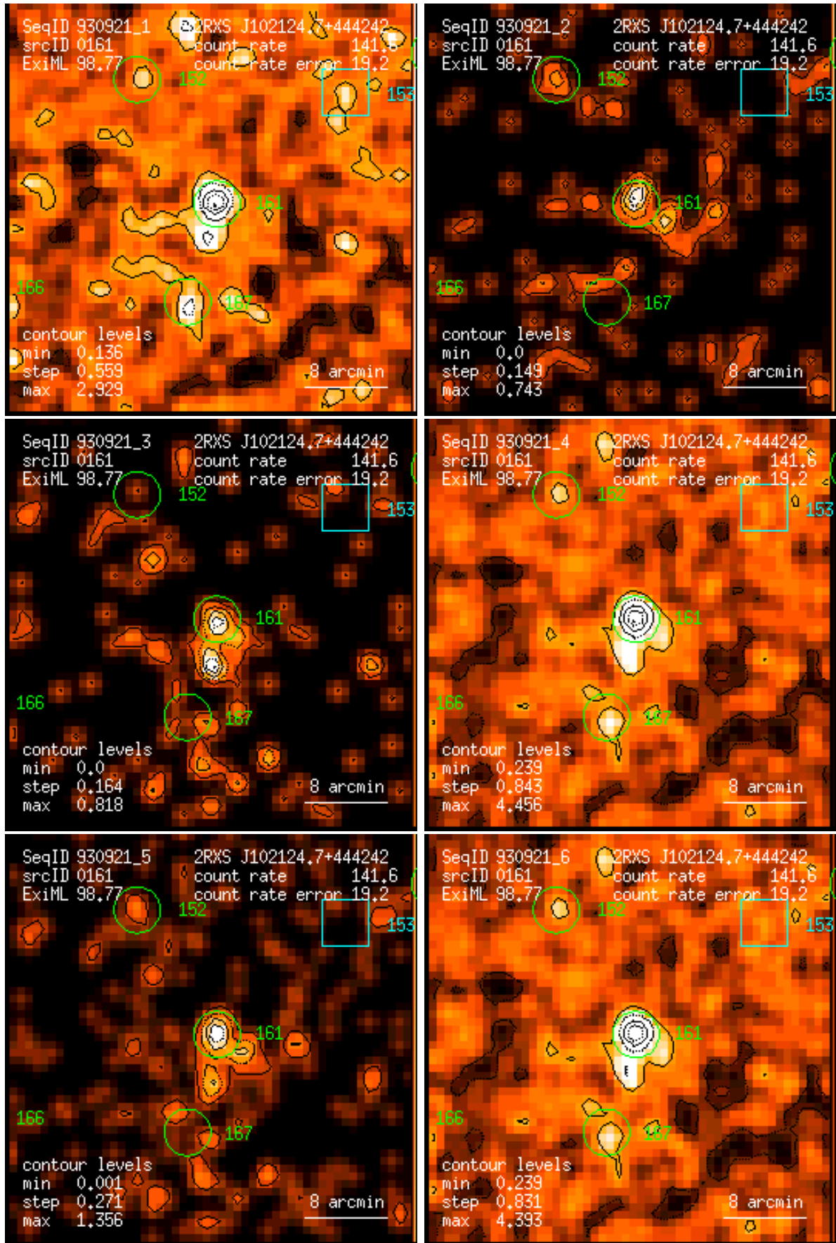
Figure 161: RASS 930921: detection 0161: band rate images, Gaussian filter: (1) PSPC channels 11 – 41, (2) 52 – 90, (3) 91 – 201, (4) 11 – 235, (5) 52 – 201, (6) 11 – 201. Broad band rates in counts/ks. Band rate contour levels in counts/ks/arcmin 2 .
