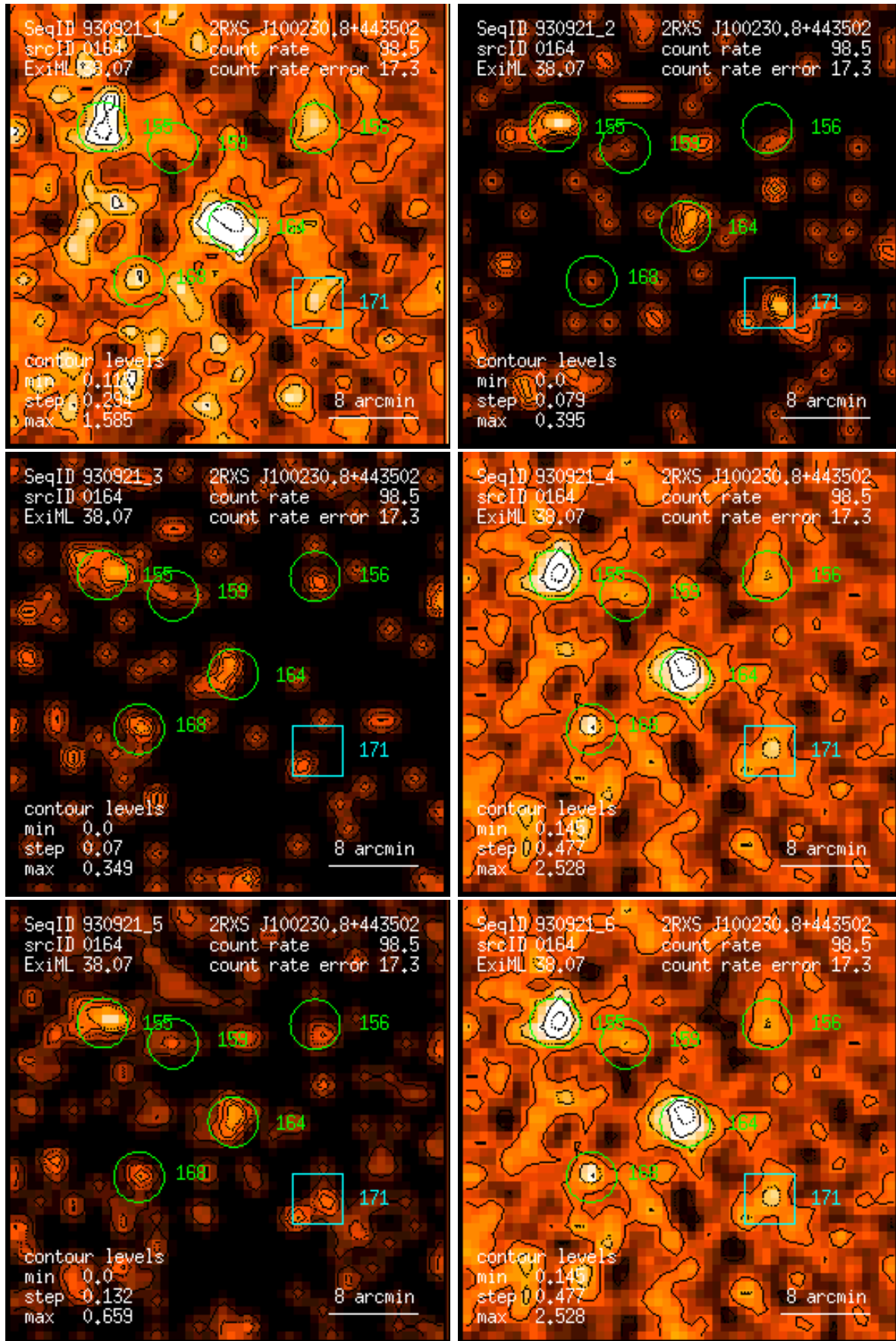
Figure 164: RASS 930921: detection 0164: band rate images, Gaussian filter: (1) PSPC channels 11 – 41, (2) 52 – 90, (3) 91 – 201, (4) 11 – 235, (5) 52 – 201, (6) 11 – 201. Broad band rates in counts/ks. Band rate contour levels in counts/ks/arcmin 2 .
