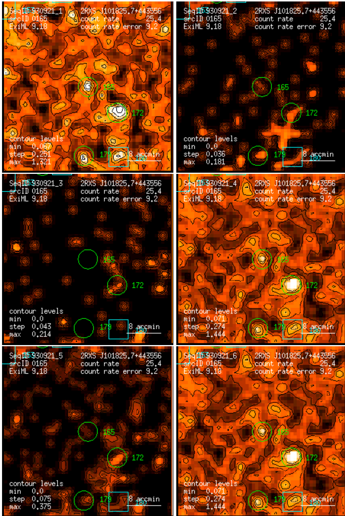
Figure 165: RASS 930921: detection 0165: band rate images, Gaussian filter: (1) PSPC channels 11 – 41, (2) 52 – 90, (3) 91 – 201, (4) 11 – 235, (5) 52 – 201, (6) 11 – 201. Broad band rates in counts/ks. Band rate contour levels in counts/ks/arcmin 2 .
