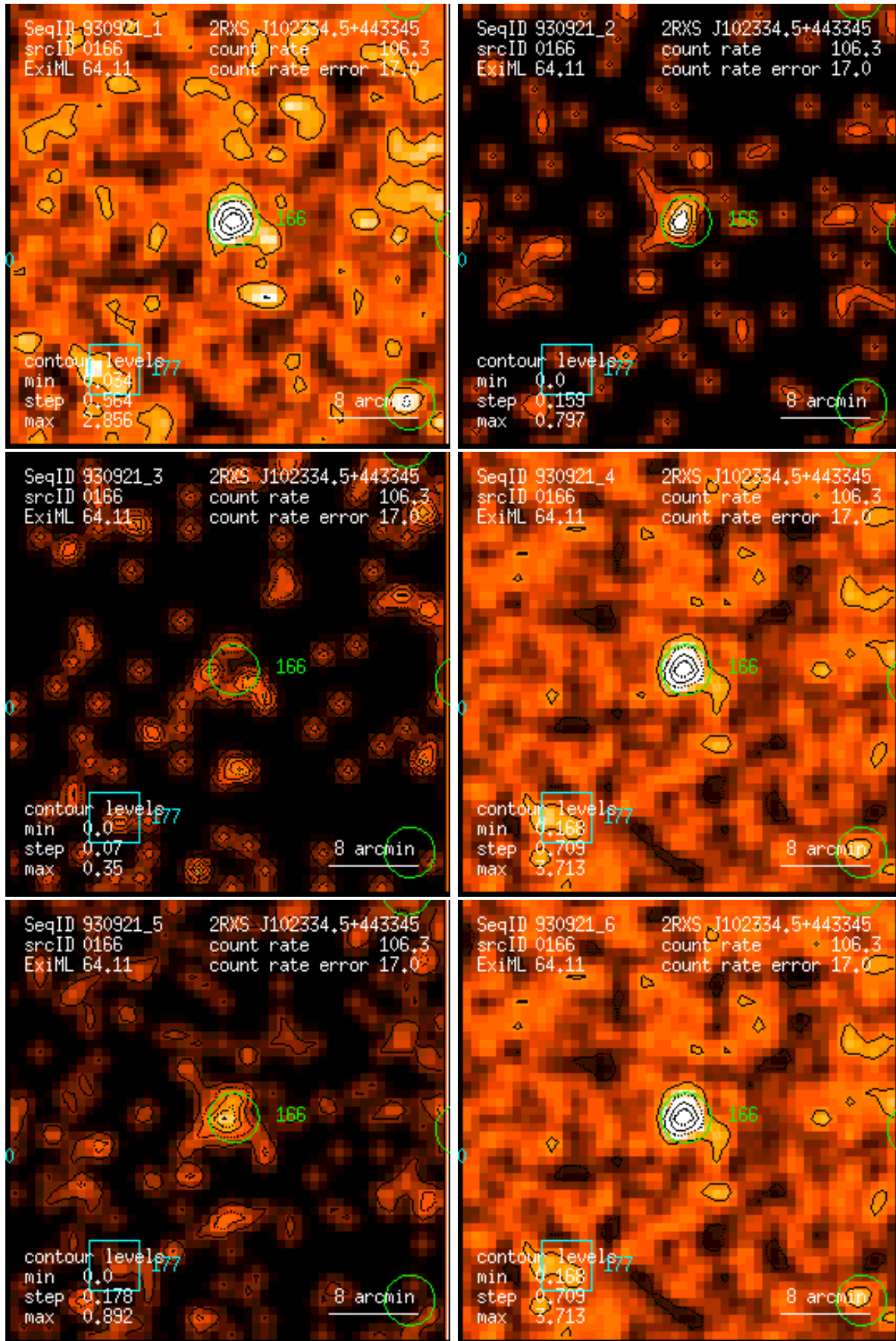
Figure 166: RASS 930921: detection 0166: band rate images, Gaussian filter: (1) PSPC channels 11 – 41, (2) 52 – 90, (3) 91 – 201, (4) 11 – 235, (5) 52 – 201, (6) 11 – 201. Broad band rates in counts/ks. Band rate contour levels in counts/ks/arcmin 2 .
