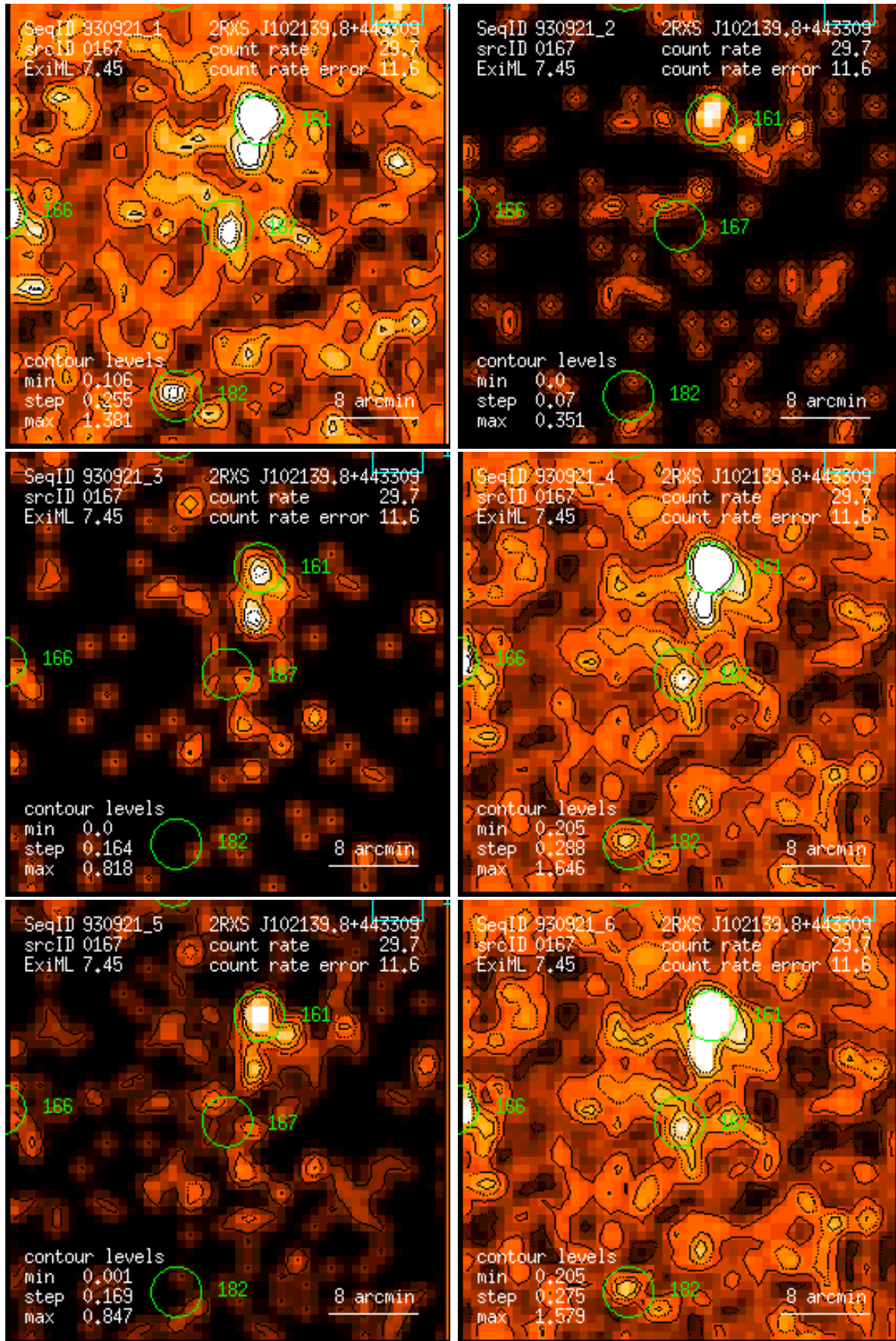
Figure 167: RASS 930921: detection 0167: band rate images, Gaussian filter: (1) PSPC channels 11 – 41, (2) 52 – 90, (3) 91 – 201, (4) 11 – 235, (5) 52 – 201, (6) 11 – 201. Broad band rates in counts/ks. Band rate contour levels in counts/ks/arcmin 2 .
